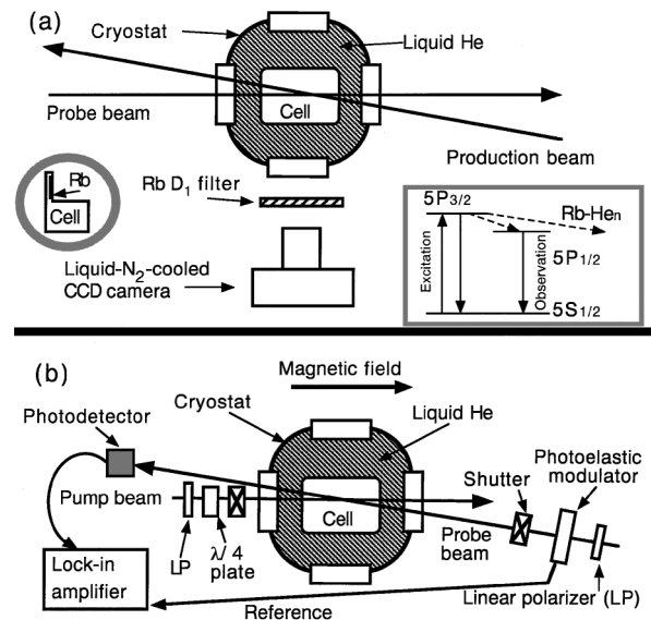
FIG. 1. Experimental setups (a) for monitoring Rb atoms by D_1 fluorescence imaging, and (b) for measuring the spin relaxation of optically polarized Rb atoms. The schematic figure of the cell is depicted inside circle in (a). The energy-level diagram of Rb related to D_1 fluorescence imaging is shown in the inset in (a). The production beam is not displayed in (b).
