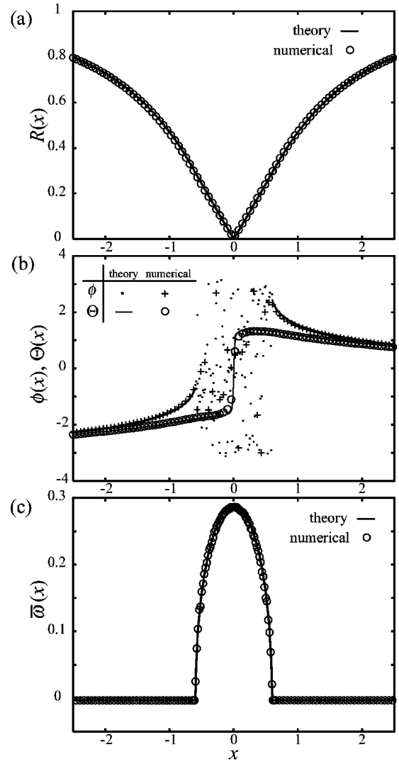
FIG. 6. Comparison between the theory and numerical simulation. Theoretical results are indicated with solid lines in (a) and (c), and solid lines and scattered dots in (b). Numerical data, which are the same as those given in Fig. 5, are indicated with open circles and crosses. (a) Instantaneous radial profile of the mean-field modulus R . (b) Instantaneous radial profile of the mean-field phase \Theta and that of the phases \phi of the local oscillators, where the theoretically obtained scattered dots are the random numbers chosen from the probability distribution given by Eq. (16). (c) Radial profile of the mean frequency \bar{\omega} of the local oscillators.
