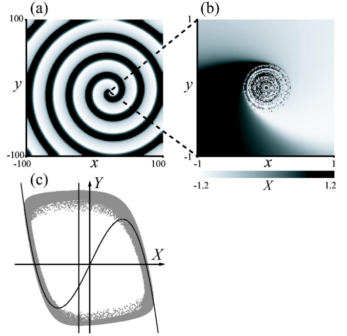
FIG. 2. Spiral patterns exhibited by nonlocally coupled FitzHugh-Nagumo oscillators with K=2.0 , presented in a similar manner to Fig. 1. For this value of K , the amplitude degrees of freedom become almost irrelevant.
