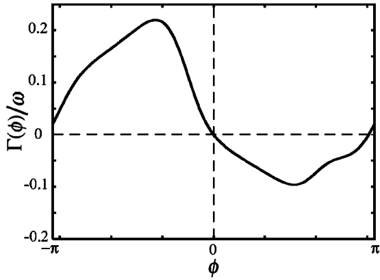
FIG. 3. Phase-coupling function \Gamma(\phi) vs \phi for coupled FitzHugh-Nagumo oscillators. This quantity can be used for the study of nonlocally coupled phase oscillators given by Eq. (10).
