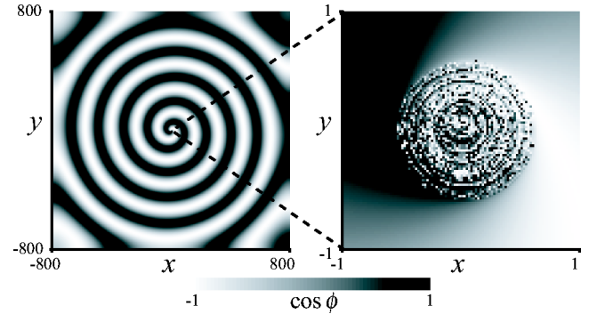
FIG. 4. Spiral pattern (left) and its core structure (right) exhibited by nonlocally coupled phase oscillators governed by Eq. (11), where \alpha=0.3 .
