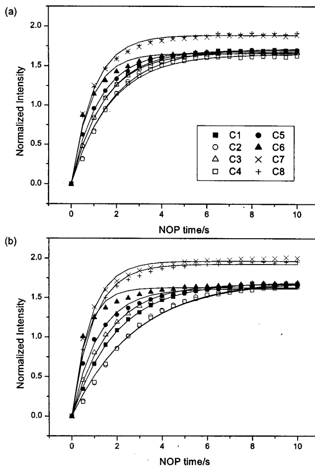
FIG. 4. NOP time dependence of the area intensities of the ^{13}\text{C} signals in uniformly ^{13}\text{C} , ^{15}\text{N} -labeled glycyloisoleucine. DARR irradiation ( \nu_1 = \nu_{\text{MAS}} = 20 kHz) was applied for (a), while \nu_1 = 5 kHz for (b). Each signal intensity is given by taking the corresponding area intensity observed by a ^{13}\text{C} 90^\circ pulse with a relaxation interval of 300 s as 1.0. The solid lines are the best-fit curves to Eq. (10) with the best-fit parameters collated in Table I.
