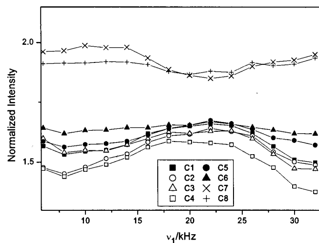
FIG. 6. DARR rf-strength dependence of the intensities of the signals of uniformly ^{13}\text{C} , ^{15}\text{N} -labeled glycylisoleucine at \nu_{\text{MAS}} = 20 kHz. Each signal is normalized to the corresponding area intensity observed by a ^{13}\text{C} 90^\circ pulse with a relaxation interval of 300 s. The solid lines are for eye-guidance.
