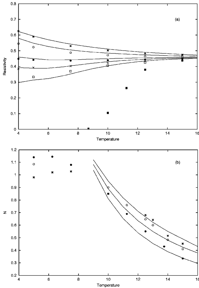
FIG. 1. (a) Resistivity \rho ( \text{m}\Omega \text{ cm} ) and (b) Nernst coefficient N ( \mu\text{V}/\text{K} ) data in LSCO x=0.06 (Ref. 23) in 2 (open square), 3 (cross), 4 (closed circle), 6 (open circle), and 8 (asterisk) (T) at each T (K) and the corresponding theoretical (solid) curves. The parameter values used are \lambda(0)=2.3 ( \mu\text{m} ), H_0=493 (T), T_{c0}=13 (K), s=1.5 (nm), and T_0=96 (K).
