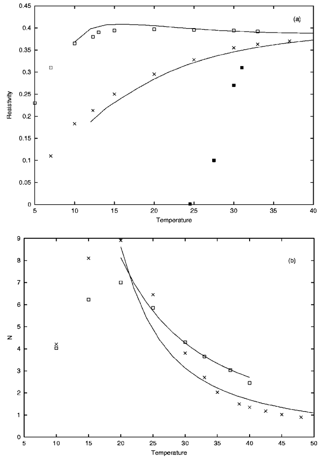
FIG. 2. Corresponding results to Fig. 1 for LSCO x=0.08 (Ref. 12) in 12 and 26 (T). The parameter values are \lambda(0)=0.43 ( \mu\text{m} ), H_0=235 (T), T_{c0}=32 (K), s=1.5 (nm), and T_0=96 (K).
