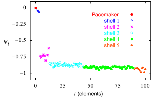
FIG. 1 (color online). Phases of elements in the entrained state; N = 100 , p = 0.05 , N_1 = 3 , \kappa = 100 , and \mu = 1000 .
