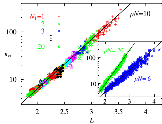
FIG. 2 (color online). Dependence of the entrainment threshold on the depth L for an ensemble of random networks with N = 100 and p = 0.1 . In the inset, respective data for networks with p = 0.06 and 0.2 are plotted. Solid lines are the exponential functions c_p(1 + pN)^L with appropriate fitting parameters c_p .
