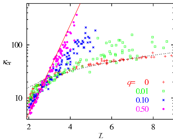
FIG. 3 (color online). Dependence of the entrainment threshold on the depth L for an ensemble of small-world networks with N = 100 , k = 3 , various N_1 , 1 \leq N_1 \leq 20 , and different randomness q . The solid line is the same exponential function as that fitted to the data with pN = 6 (= 2k) in Fig. 2. The dotted line is linear fitting for the regular lattice ( q = 0 ).
