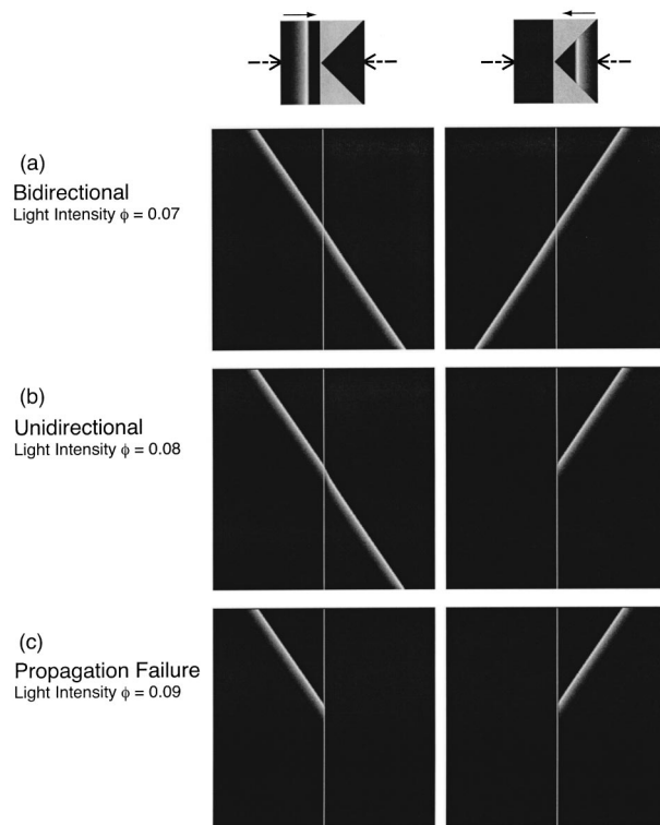
FIG. 8. Computer simulation of the manner of wave propagation with the same spatial geometry as in Fig. 7. Space-time plot of traveling waves with the variable \nu in Eqs. (1)–(3) along the horizontal centerline of the diode geometry (750 points).
