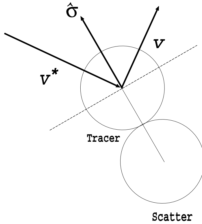
FIG. 1. Unit vector \hat{\sigma} pointing from the center of a scatter to the center of a tracer. The pre-collision velocity of the tracer and the post-collision velocity of it are expressed as \mathbf{v}^* and \mathbf{v} , respectively.
