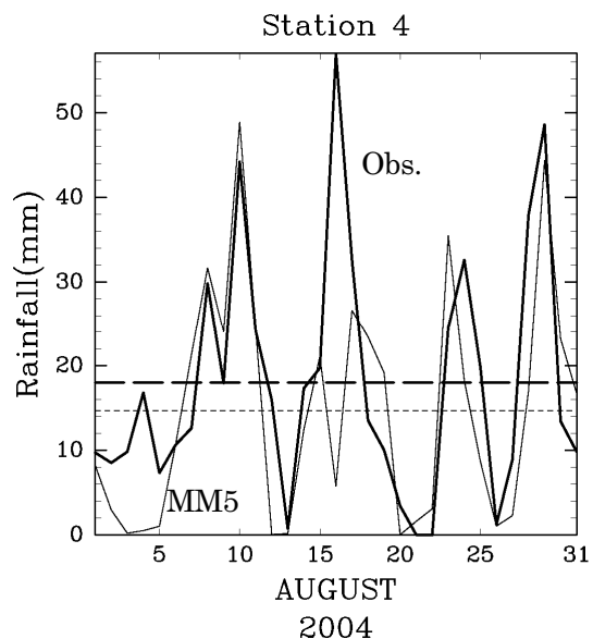
Fig. 6 Day-to-day variations of the daily rainfall in August 2004 at Station No. 4 for the two datasets: observation (thick solid line) and the MM5 output (thin solid line).
