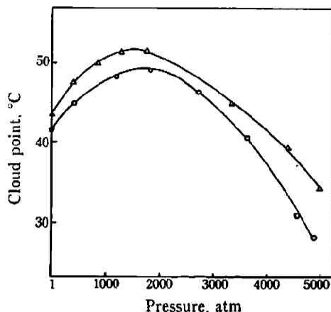
Fig. 4 Effect of pressure on the cloud point of polyoxyethylene nonylphenyl ether ( C_9H_{19}C_6H_4O(CH_2CH_2O)_{8.3}H —water —○—: 0.05 wt% —△—: 10.0 wt%
