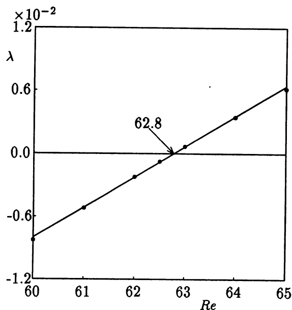
Fig. 7 Linear growth rate \lambda, r_1 = 1 .
