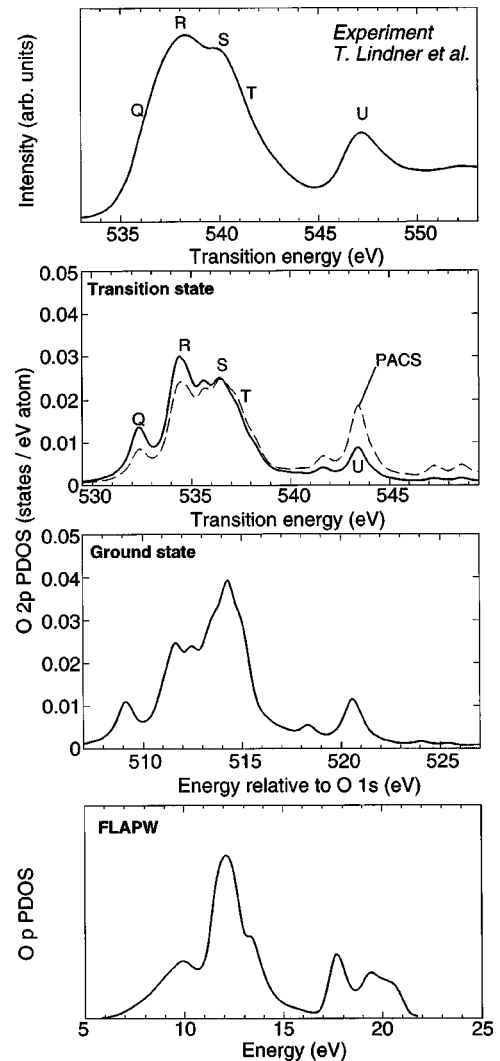
FIG. 3. (From top to bottom) Experimental O K -edge ELNES of MgO by Lindner et al. (Ref. 13). Theoretical O 2p PDOS by a cluster (O_{63}Mg_{62})^{2-} calculated for Slater's transition state and for the ground state. O p PDOS by the FLAPW band-structure calculation.
