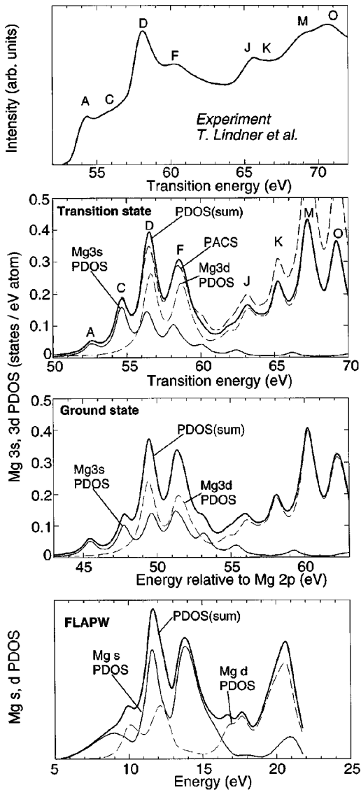
FIG. 2. (From top to bottom) Experimental Mg L_{2,3} -edge ELNES of MgO by Lindner et al. (Ref. 13). Theoretical Mg 3s, 3d PDOS by a cluster (Mg_{61}O_{62})^{2+} calculated for Slater's transition state and for the ground state. Mg s and d PDOS by the FLAPW band-structure calculation.
