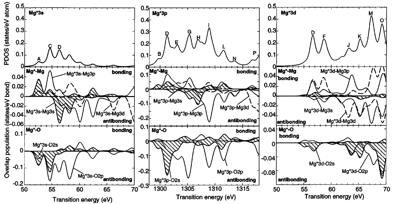
FIG. 4. Unoccupied PDOS of Mg^* 3s (left), Mg^* 3p (center), and Mg^* 3d (right) by a cluster (Mg_{63}O_{62})^{2+} for Slater's transition state, and their related overlap-population diagrams. Mg^* denotes the core-hole Mg atom. In the overlap-population diagrams of Mg^*-Mg (second row), the Mg^*-Mg 3s , and Mg^*-Mg 3p and Mg^*-Mg 3d contributions are shown by the hatched area, solid curve, and broken curves, respectively. Because of the presence of the core hole, Mg^* 3s-Mg 3p and Mg^* 3p-Mg 3s are not the same, for example. In the overlap-population diagrams of Mg^*-O (third row), Mg^*-O 2s and Mg^*-O 2p are shown by the hatched area and solid curve.
