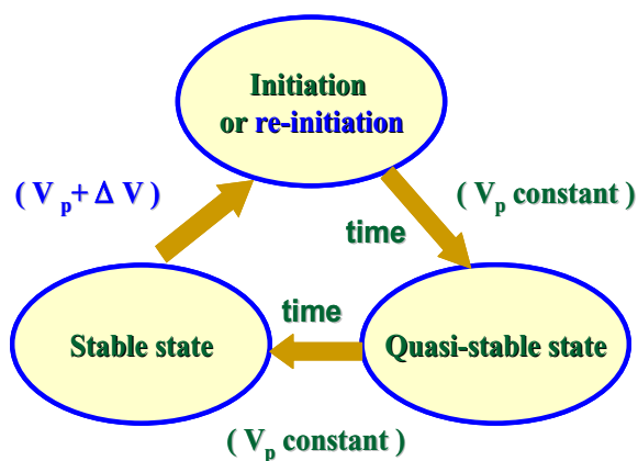
Figure 1. Charging process under ac voltage excitation in vacuum.
