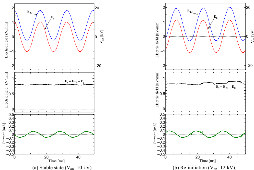
Figure 5. Different charging states for an insulator with comparatively rough surface. (Pyrex®, R_a=0.75 \mu\text{m} )
