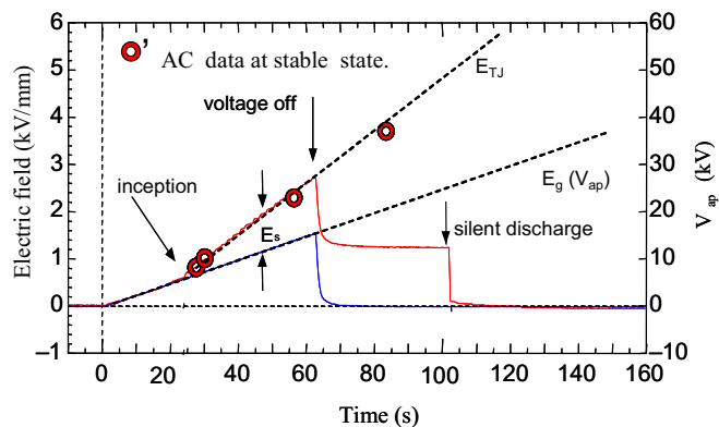
Figure 6. Typical charging process when an insulator is subjected to a ramped dc voltage. (PMMA, R_a = 0.17 \mu\text{m} . The stable state is established at this roughness.)
