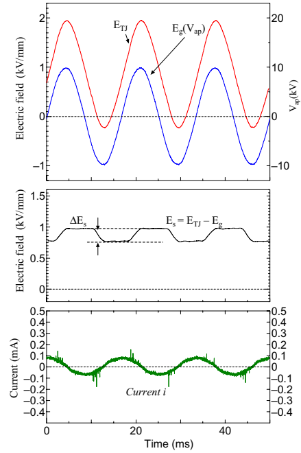
Figure 4. Wave forms of probe signal and current when the charging has reached at quasi-stable state.
