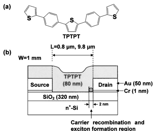
FIG. 1. (a) Molecular structure of TPTPT, (b) structure of organic light-emitting field-effect transistor (OLEFET). The area of carrier recombination and exciton formation used in the calculation of light out-coupling efficiency is indicated by a circle.
