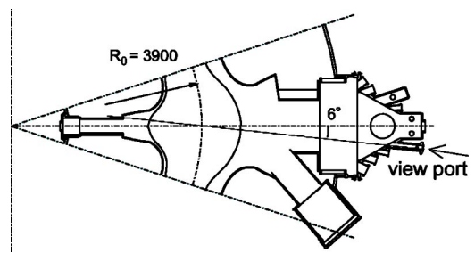
FIG. 3. Top view of 1-O port of the LHD. Dotted line shows the line of sight into the plasma.
