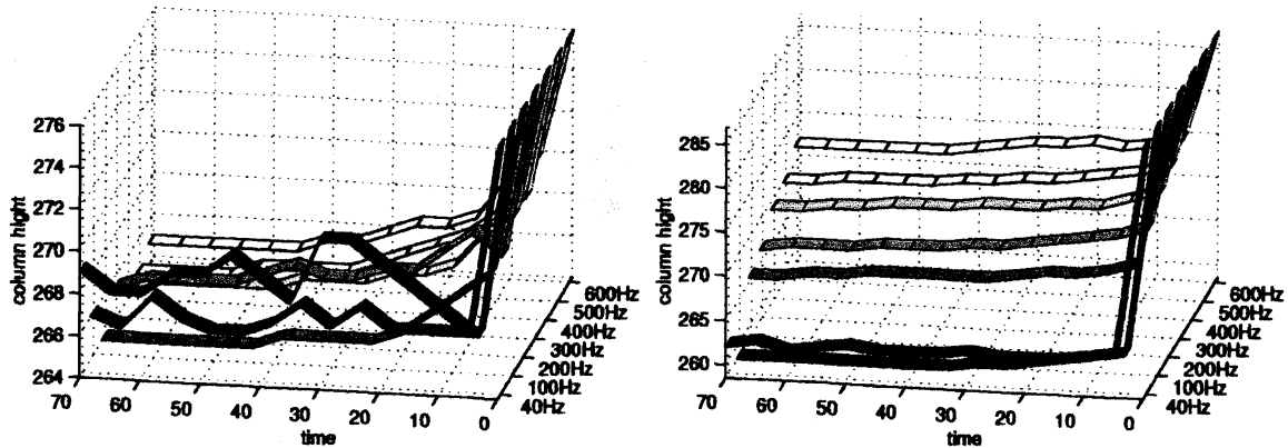
Figure 6: Compaction for spherical (left) and non-spherical particles (right), as indicated by the height of the granular column
