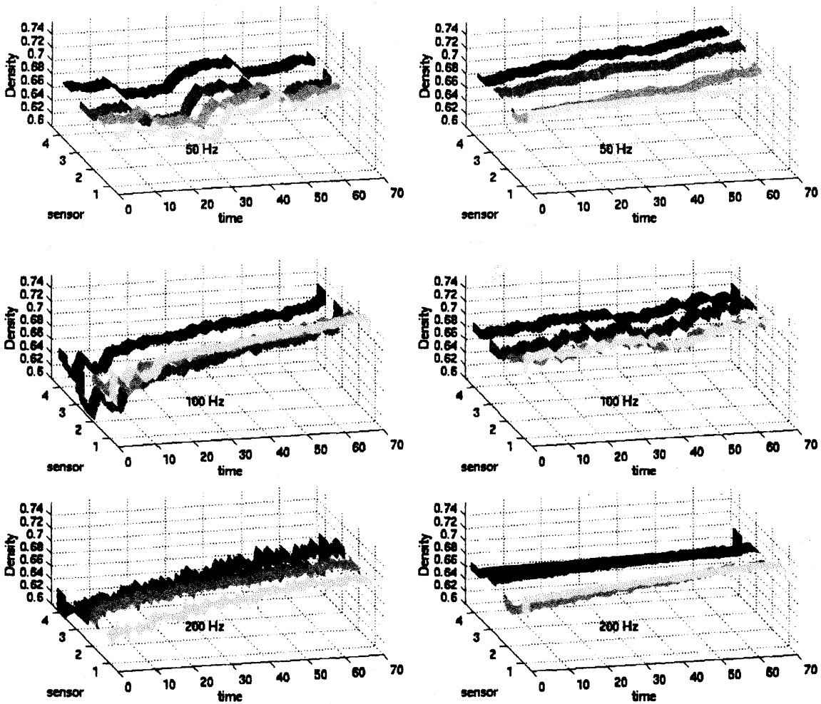
Figure 11: Continuous density response for non-spherical glass beads for initially low (left) and high (right) density with moving averages of 200 measurement points. .
