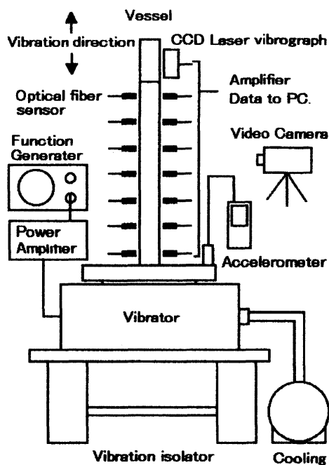
Figure 2: Full setup the effect of subtle changes in the setup.
