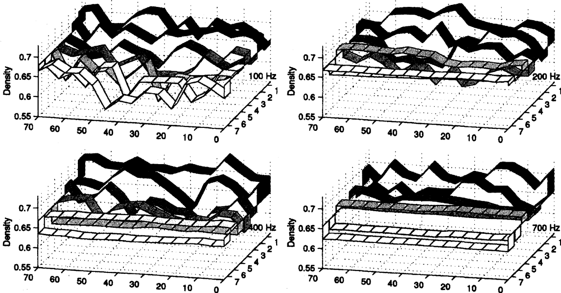
Figure 7: Density response for spherical glass beads with an average density of \rho = 0.66 , for all seven sensors (x-axis) between 0 and 70 seconds (z-axis).
