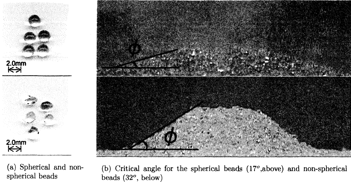
Figure 3: Shape and critical angle for spherical and non-spherical (but still convex) beads used in the experiments
