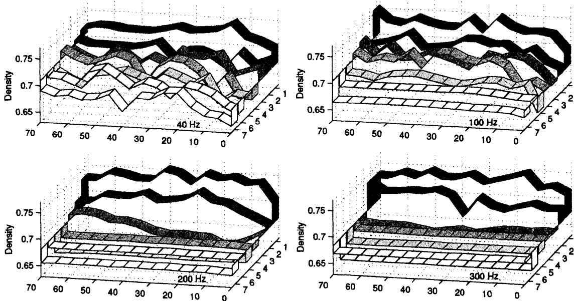
Figure 10: Density response for non-spherical glass beads with an average density of 0.68.
