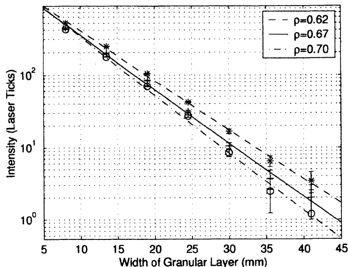
(a) Calibration-curve for the non-spherical beads; Error bars for four independent measurements
