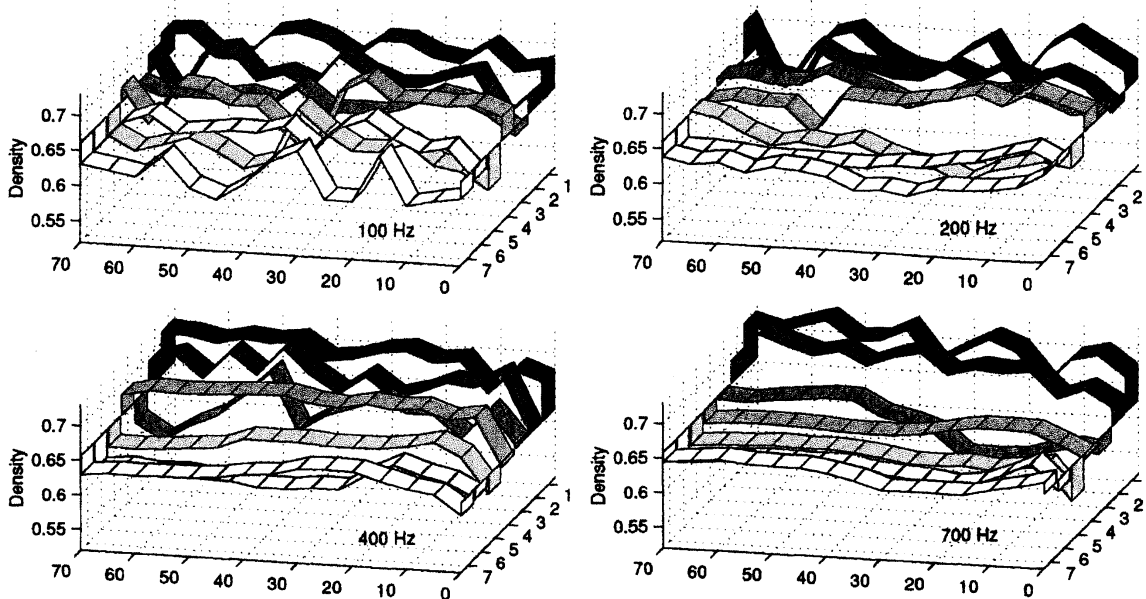
Figure 8: Density response for spherical glass beads with an average density of \rho = 0.62 , for all seven sensors (x-axis) between 0 and 70 seconds (z-axis).
