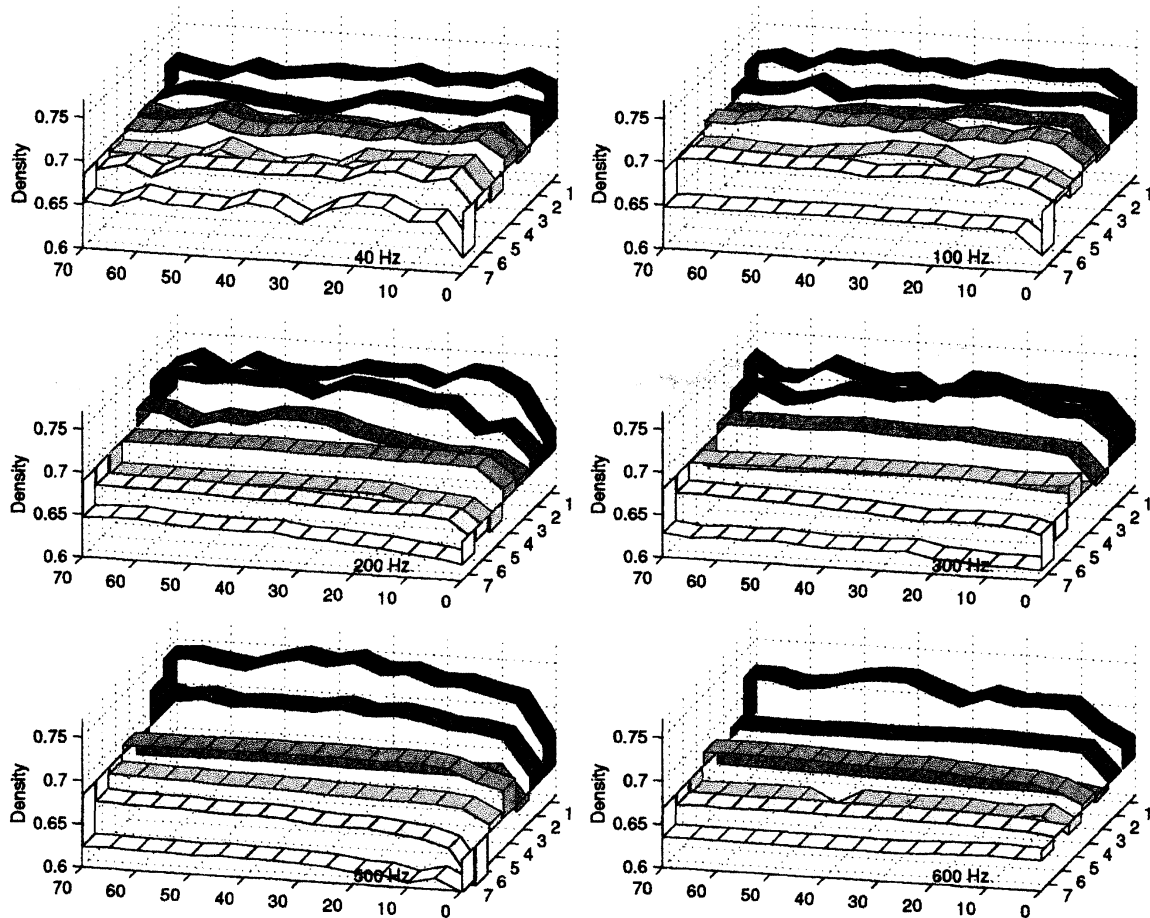
Figure 9: Density response for non-spherical glass beads with an average density of 0.61.
