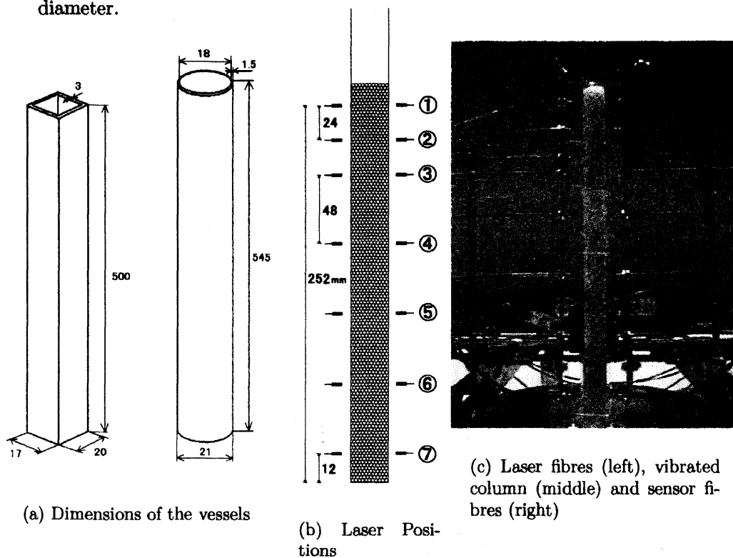
Figure 1: Dimensions of the setup
