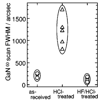
FIG. 3. Full widths at half maximum of x-ray rocking curves for (0002) diffraction from GaN layers grown on 6H-SiC substrates with three different pretreatments: (a) the as-received substrate, (b) the HCl-treated substrate and (c) the HF/HCl-treated substrate. The GaN layer grown on the HCl-treated substrate exhibits considerably wider peaks compared to the others.
