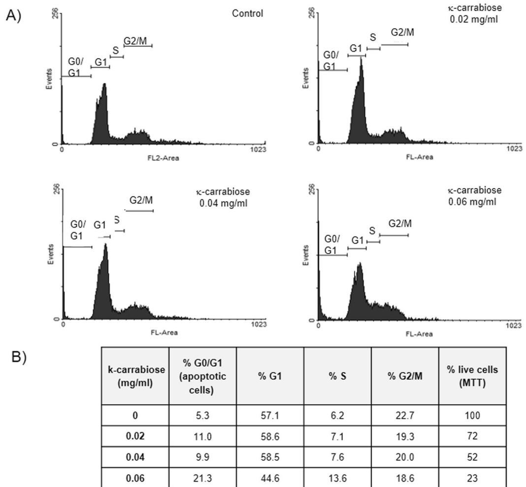
Figure 4. Influence of \kappa -carrabiose on LM2 cell cycle. LM2 cells were incubated with \kappa -carrabiose, at different concentrations, during 48 h and afterwards, the DNA was stained with propidium iodide and cell cycle was analyzed by flow cytometry as described in Materials & Methods. (A) The histograms show the number of cells (events) in each phase of the cell cycle. FL-area denotes propidium iodide fluorescence; (B) the Table shows the percentage of cells in each phase of the cycle and the correlation with the number of living cells determined by the MTT assay.
