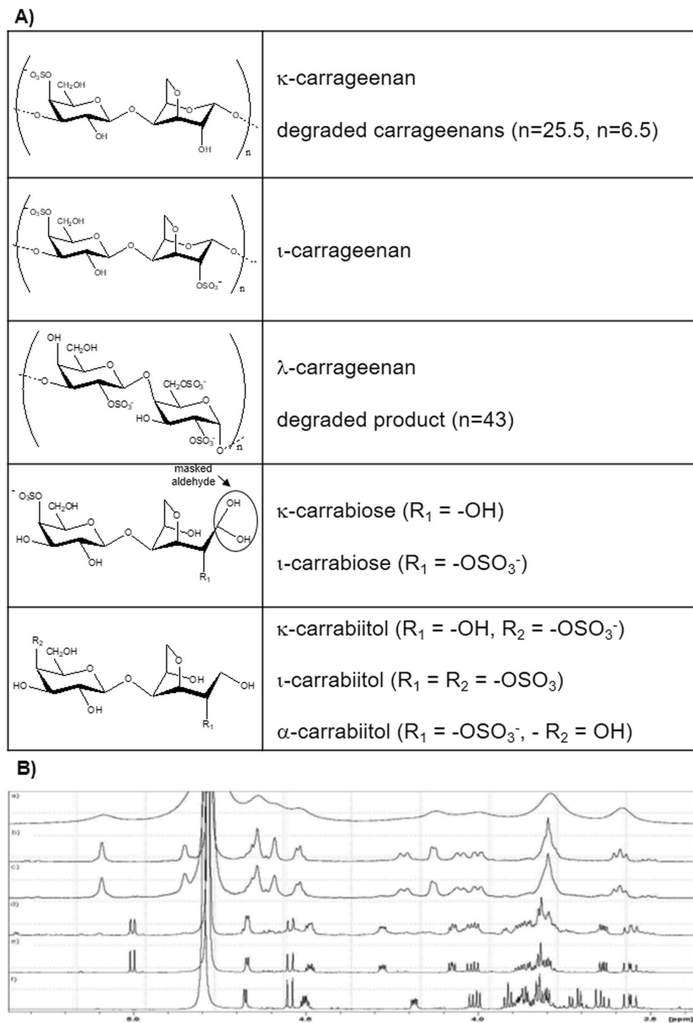
Figure 2. Polysaccharides, oligosaccharides and disaccharides: structures and characterization. (A) Chemical structures of \kappa -carrageenan and its degraded product, \iota -carrageenan, \lambda -carrageenan and its degraded product, \kappa -carrabiose, \iota -carrabiose, \kappa -carrabiitol, \iota -carrabiitol and \alpha -carrabiitol. (B) 500 MHz ^1\text{H-NMR} spectra of \kappa -carrageenan and its oligosaccharides in \text{D}_2\text{O} : (a) undegraded \kappa -carrageenan, (b) degraded \kappa -carrageenan ( n = 25.5 ), (c) degraded \kappa -carrageenan ( n = 6.5 ), (d) impure \kappa -carrabiose, (e) \kappa -carrabiose, and (f) \kappa -carrabiitol.
