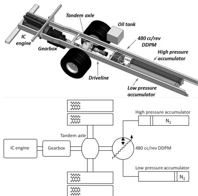
Fig.5 Simplified layout of a parallel hydraulic braking energy recovery system.
