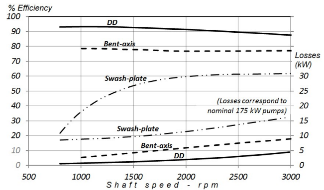
Fig.2 As Figure 1, but with pumps at 20% displacement.
