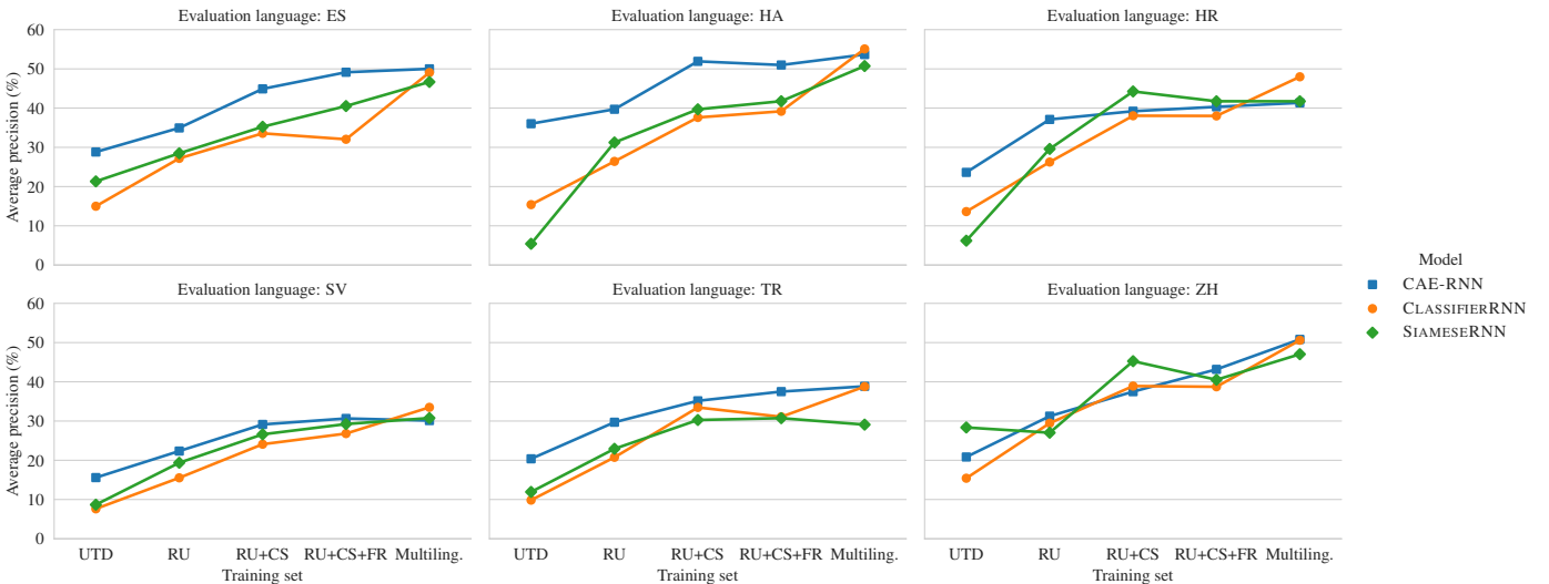
Fig. 4. AP (%) on development data for the six zero-resource language, as multilingual models are trained on one (RU), two (RU+CS), three (RU+CS+FR) and all six (multiling.) training languages. Scores from unsupervised models trained on UTD segments from the evaluation language are also given.
