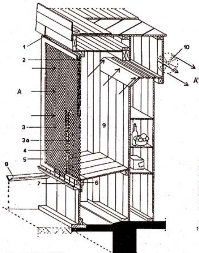
13. Air cooler 1:50
