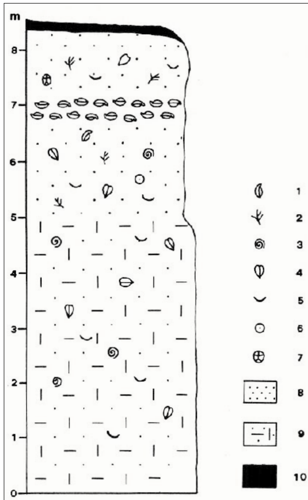
Figure 3. Albanese quarry, stratigraphical succession of lower Pleistocene calcarenites and sands; (1) Terebratula scillae ; (2) Bryozoa; (3) Gastropods; (4) Pelecypods; (5) Pectinids; (6) Regular echinoids; (7) Irregular echinoids; (8) Sands; (9) Calcarenites; (10) Soil.
