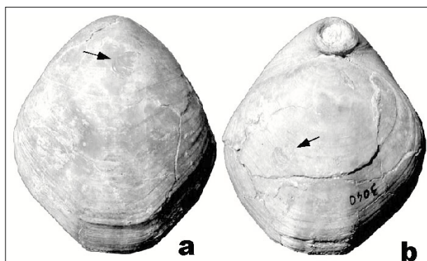
Figure 5. Terebratula scillae , specimen n° 3040, 7.5 cm in length; pedicle (a) and brachial (b) valve, both exhibiting Centrichnus eccentricus .
