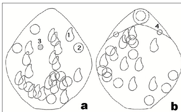
Figure 6. Trace position on the pedicle (a) and brachial (b) valves of Terebratula scillae . (1) Centrichnus eccentricus ; (2) Podichnus centrifugalis ; (3) Oichnus simplex ; (4) Oichnus isp.
