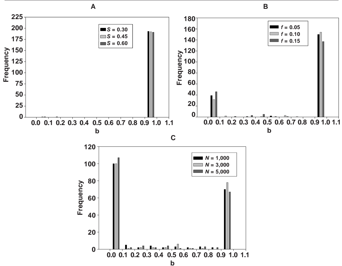
Fig. 1. Example frequency distributions of ultra-power model estimator for: A. \rho_{Sf} = -0.90 , conditional on \mu_S(S) ; B. \rho_{Sf} = -0.45 , conditional on \mu_f ; C. \rho_{Sf} = 0.00 , conditional on N .
