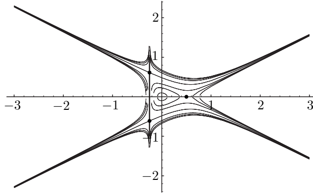
Figure 5. Phase portrait of differential system (15) for parameters \alpha = 2 , \gamma = 2 and \beta = 1 - \alpha = -1 .
