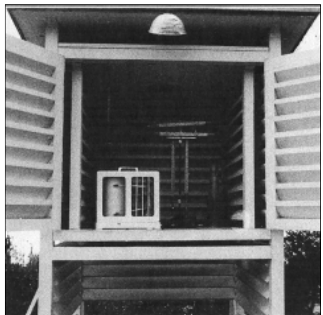
Figure 10. A meteorological shelter showing some of the instruments inside. Meteorological observations began in 1913 at the Fabra Observatory and have continued without any interruption at the same site.
