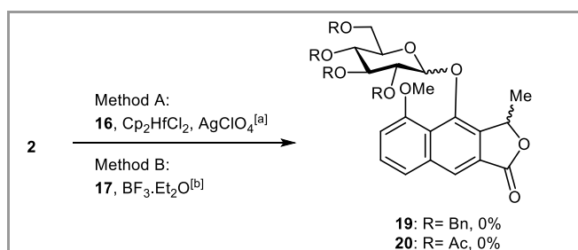
Scheme 4 Attempted O -glycosidation reaction toward the total synthesis of eleuthoside A ( 1 ); comparative studies for the attachment of the floride and imidate sugar donors. [a] Method A: 16 (0.5 eq.), Cp 2 HfCl 2 (0.5 eq.), AgClO 4 (1 eq.), MS 4A, CH 2 Cl 2 , -70 °C- rt, 1 or 24 h. [b] Method B: 17 (2 eq.), BF 3 ·Et 2 O (0.2 eq.), MS 4A, CH 2 Cl 2 , -10 °C- rt, 24 h.
