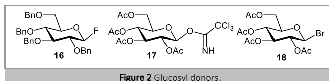
Figure 2 Glycosyl donors.
