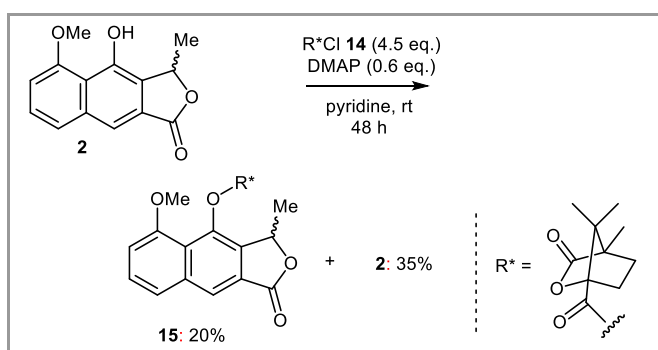
Scheme 3 Unsuccessful optical resolution protocol of eleutherol ( 2 ).
