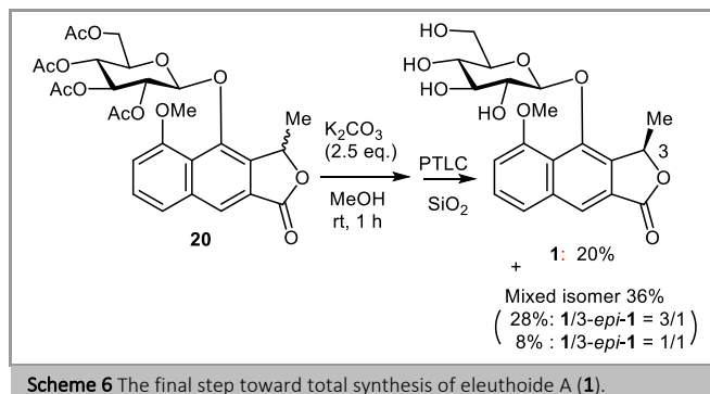
Scheme 6 The final step toward total synthesis of eleuthoside A ( 1 ).
