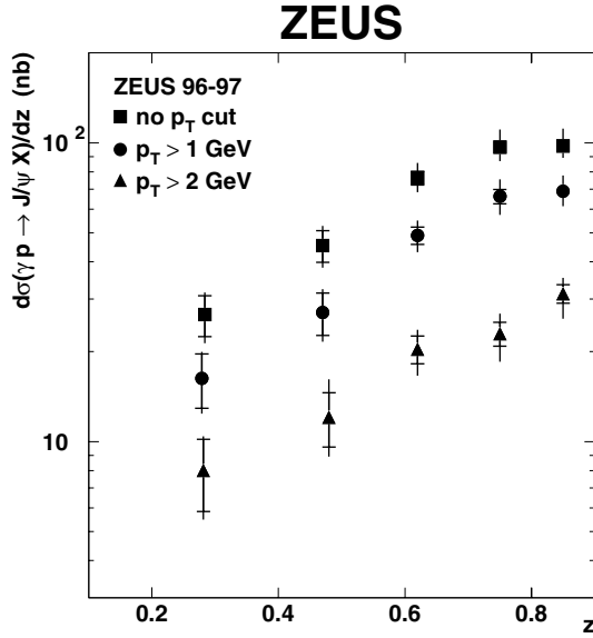
Fig. 5. Differential cross-sections d\sigma/dz for 50 < W < 180 GeV and different p_T selections: no p_T cut ( squares ), p_T > 1 ( circles ), and p_T > 2 GeV ( triangles ). The inner error bars show the statistical uncertainty; the outer bars show the statistical and systematic uncertainties added in quadrature
