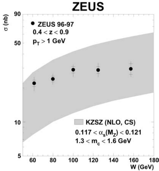
Fig. 7. Cross section as a function of W for p_T > 1 GeV and 0.4 < z < 0.9 . The inner error bars show the statistical uncertainty; the outer bars show the statistical and systematic uncertainties added in quadrature. The shaded band shows the prediction KZSZ (NLO, CS). The spread in the prediction is due to uncertainties on the charm-quark mass and on the QCD scale parameter, \Lambda_{QCD} . A 15% contribution has been added to the prediction to account for J/\psi mesons originating from \psi' cascade decays
