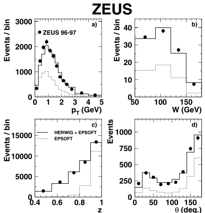
Fig. 3a–d. Number of events reconstructed in the kinematic region z > 0.4 and 50 < W < 180 GeV plotted against a J/\psi p_T , b W , c inelasticity, z and d J/\psi polar angle, \theta . The data distributions are shown as the points with statistical errors only. The simulated EPSOFT diffractive proton-dissociation background is shown as the dotted lines. The solid lines show the prediction of the sum of the HERWIG and EPSOFT generators. The combined MC has been area normalised to the data. The HERWIG MC sample was reweighted in p_T and W to the data
