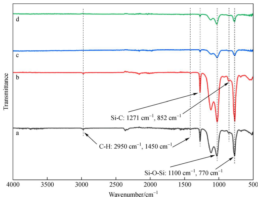
Fig. 4 FTIR spectra of MTMS-derived SAs using (a) deionized water, (b) hexane, (c) 0.044 g·mL -1 and (d) 0.022 g·mL -1 sodium bicarbonate solution in solvent exchange step, respectively.
