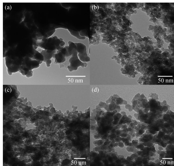
Fig. 5 TEM images of MTMS-derived SAs using in solvent exchange step (a) deionized water, (b) hexane, (c) 0.044 g·mL -1 and (d) 0.022 g·mL -1 sodium bicarbonate solution, respectively.
