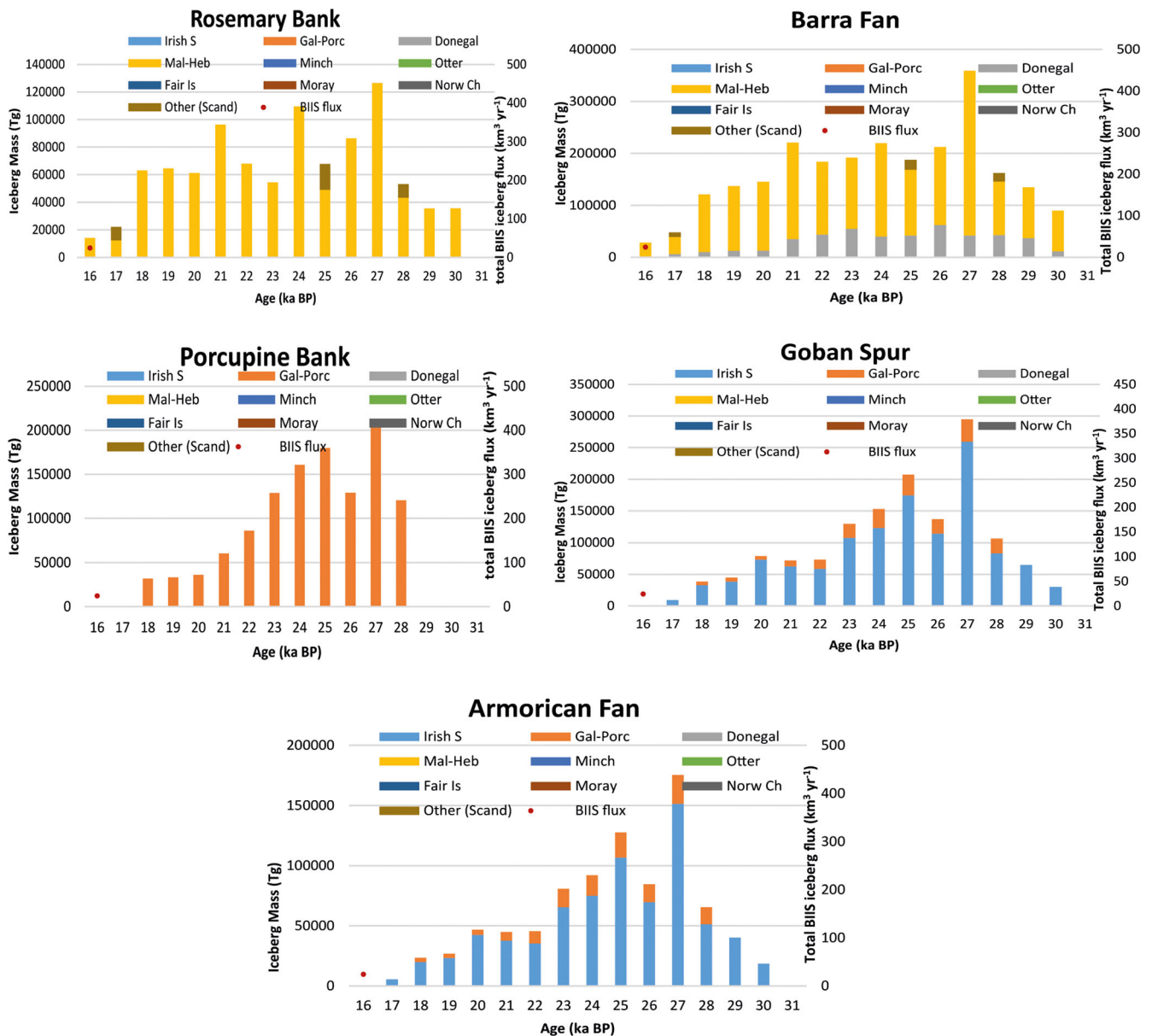
Figure 6. Bar charts of the ice-rafted debris (IRD) source variation over time within 2^\circ of the 5 IRD marine cores, using modelled iceberg mass (in Tg) as a proxy (see Table 1 for core names and locations). Note that the dotted line is the total BIIS iceberg flux (in \text{km}^3 \text{yr}^{-1} ; see right-hand scale), as reconstructed in Fig. 3. See Figs. 1 and 3 for release sites and fluxes, respectively. [Color figure can be viewed at wileyonlinelibrary.com ]
