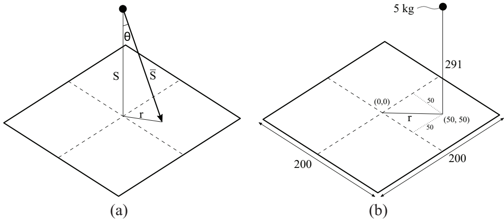
Figure 12. Experimental schematics for a spherical charge detonating above a square target: (a) general case of a centrally located charge; (b) example off-centre case of 5 kg PE4 at 291 mm normal stand-off distance, offset by 50 mm in both in-plane directions from the centre of a 200 mm square plate. Note: dimensions in mm.
