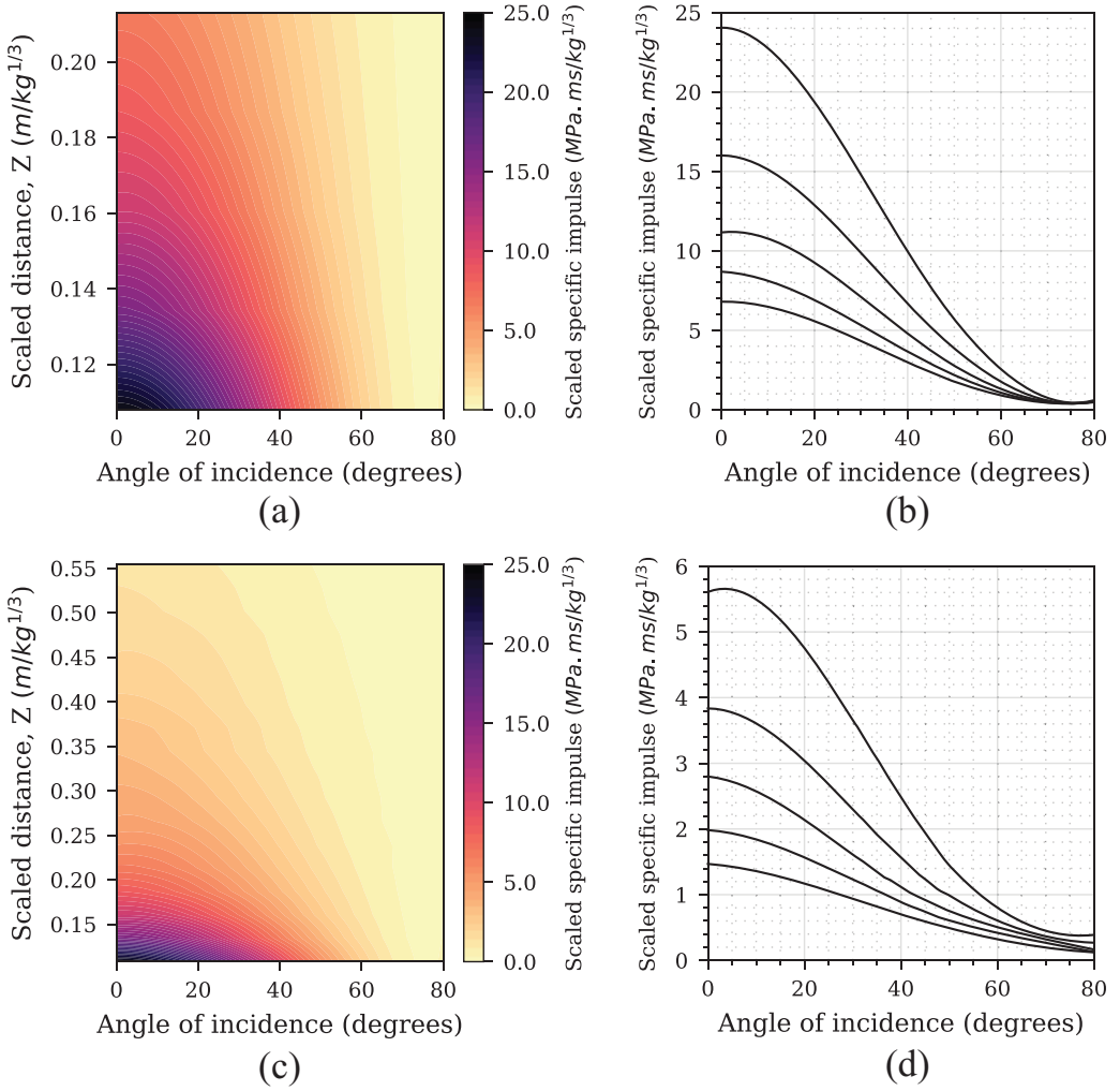
Figure 5. CFD results: (a) filled contours of scaled peak specific impulse for reduced dataset, 0.11–0.21 m/kg^{1/3} , (b) distributions of peak specific impulse for 0.11, 0.13, 0.16, 0.19 and 0.21 m/kg^{1/3} , (c) filled contours of scaled peak specific impulse for full dataset, 0.11–0.55 m/kg^{1/3} and (d) distributions of peak specific impulse for 0.24, 0.32, 0.40, 0.48 and 0.55 m/kg^{1/3} .
