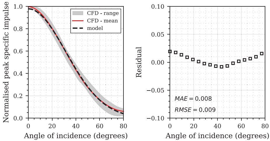
Figure 8. Normalised specific impulse distributions for full dataset (0.11–0.55 m/kg 1/3 ) with associated residuals and error assessment for the Pannell et al. (2019) Gaussian model, equation (4).
