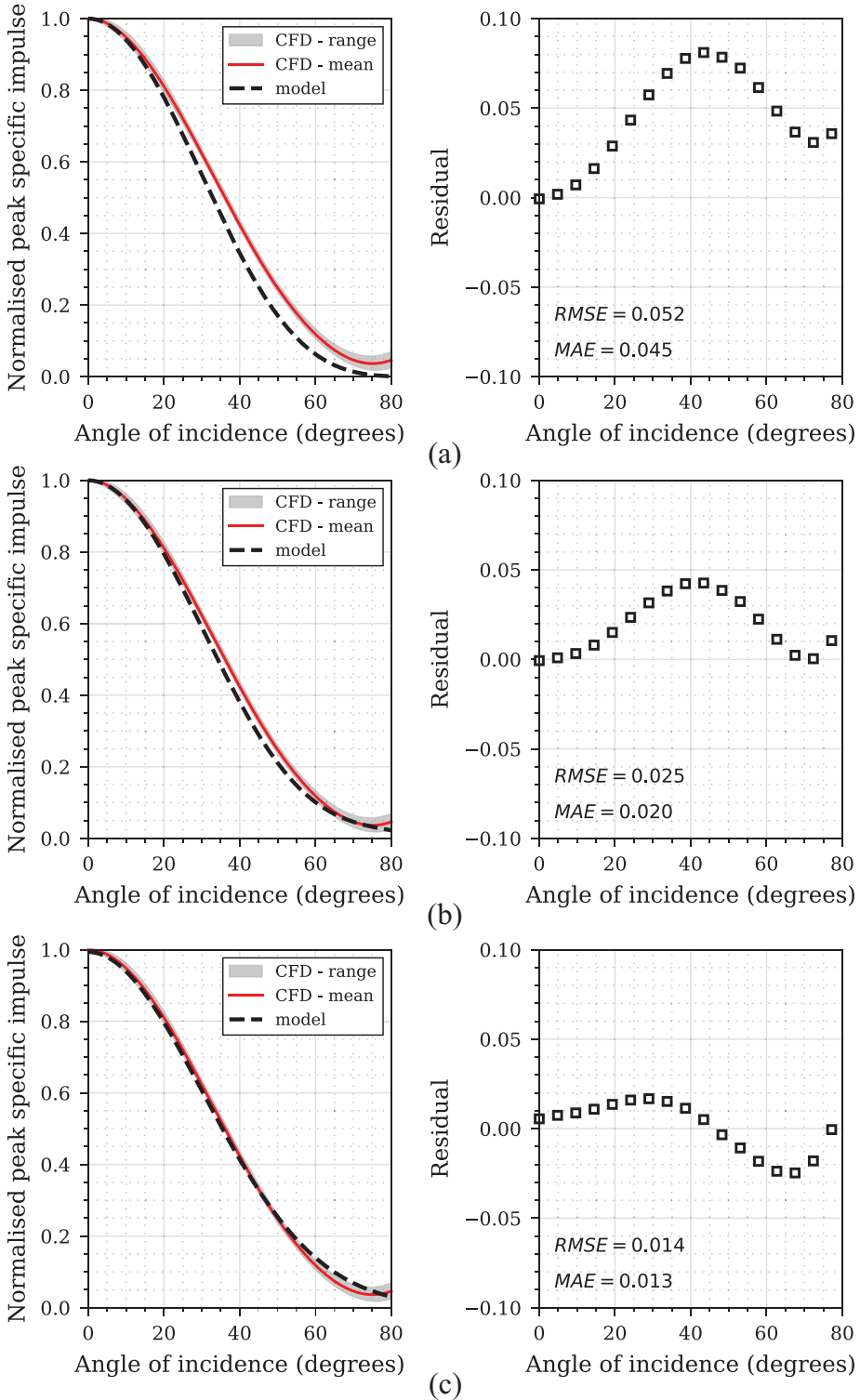
Figure 7. Normalised specific impulse distributions for reduced dataset ( 0.11\text{--}0.21\text{ m/kg}^{1/3} ) with associated residuals and error assessment: (a) Henrych (1979) trigonometric model, equation (2), (b) Randers-Pehrson and Bannister (1997) trigonometric model, equation (3) and (c) Pannell et al. (2019) Gaussian model, equation (4).
