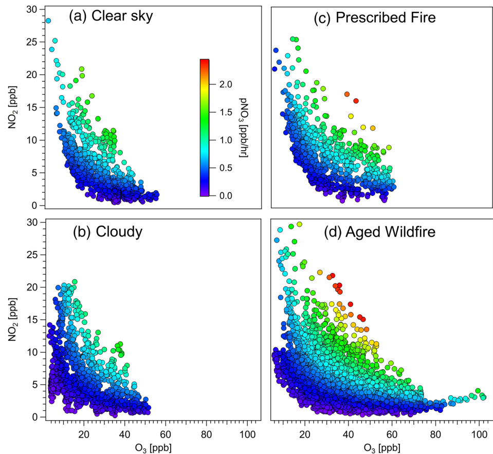
Figure 4. \text{NO}_2/\text{O}_3 plots colored by p\text{NO}_3 . Panel (a) represents typical clear sky conditions, panel (b) represents cloudy and clean conditions, panel (c) represents prescribed-fire (3 hr old) smoke conditions, and panel (d) represents aged (up to several days) wildfire smoke-impacted conditions. Points with both low \text{NO}_2 and low \text{O}_3 during smoke-impacted periods arise from \text{NO}_2 titration of \text{O}_3 and not the inclusion of clear-sky data, which was filtered out as described in section 3.
