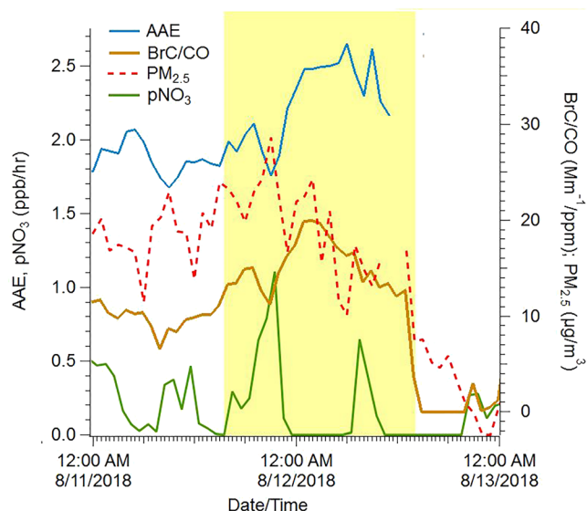
Figure 6. A likely example of nighttime, secondary BrC formation. Shortly before midnight a spike in P ( \text{NO}_3 ) occurs, followed by increases in AAE and BrC/CO as \text{PM}_{2.5} decreases, which rules out an influx of fresh smoke. These changes are consistent with increasing BrC content of the aerosol driven by reactions of \text{NO}_3 with NMOG.
