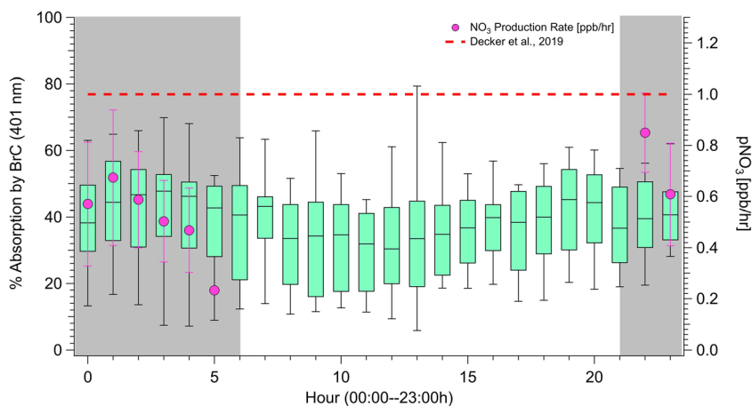
Figure 7. Hourly diurnal box and whisker plot of % absorption by BrC calculated from hourly averages of wildfire smoke-impacted 5-min data compared to the nighttime (shaded area) hourly average P ( \text{NO}_3 ). Error bars on P ( \text{NO}_3 ) represent 1\sigma .
