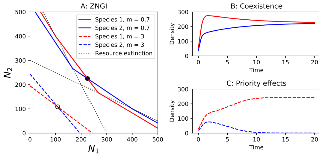
Figure B.2: A: The zero net growth isoclines (ZNGI) for the two species are shown for different mortality rates. Please note, the x and y-axis show densities of the species one and two, not as in the main text the resource densities. The species compete for a total of 4 resources, a visualisation of the ZNGI as a function of the resources is therefore not possible (4 dimensional plot). At low mortality (full lines) species reach higher equilibrium densities and two resources go extinct, as the stable equilibrium is above the resource-extinction line. The two species can stably coexist with the remaining two resources. At high mortality (dashed lines) no resources go extinct and the species compete for all resources, leading to priority effects and an unstable equilibrium. B,C: The species densities over time. Species can coexist under low mortality (B), but not under high mortality (C). The two scenarios differ only in their mortality, but as the outcome of coexistence changes from priority effects to coexistence, mortality must affect niche differences.
