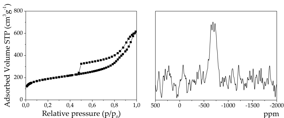
FIGURE 1.11: \text{N}_2 ads/des isotherm (left) and ^{119}\text{Sn} solid state static NMR spectrum of Sn-NTs-B (right) after the 4th cycle of the reaction of glycerol with acetone yielding solketal.
