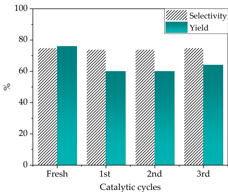
FIGURE 3.8: Recycling test of Sn-5-F127. Conditions: 100 mg of catalyst, 100 mg of DHA in 5mL EtOH, 3h at 90 °C.
