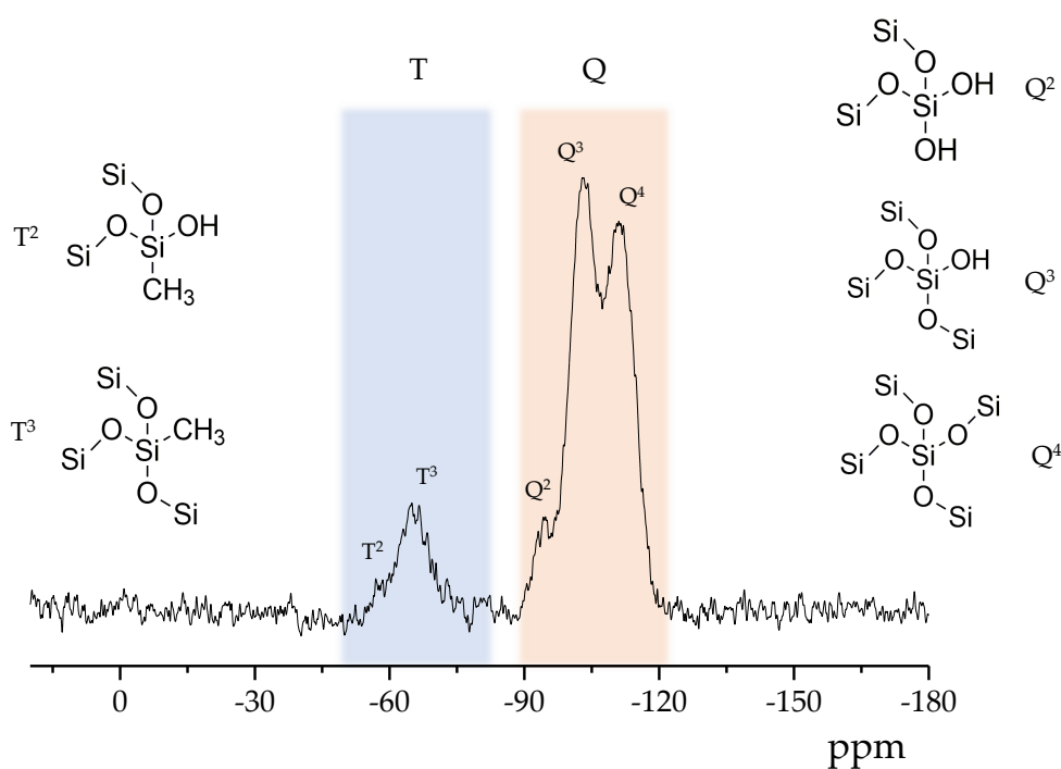
FIGURE 1.7: Direct Excitation ^{29}\text{Si} MAS NMR spectrum of a mesoporous methyl functionalized silica-based catalyst. On the right and left side, schematic representation of different silicon environments present in the bulk and on the surface.
