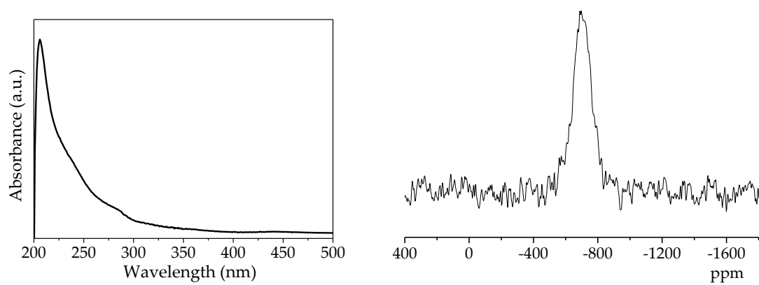
FIGURE A.2: Diffuse reflectance UV-Vis spectrum (left) and solid state ^{119}\text{Sn} static NMR spectrum (right) of SnSi-37 catalyst
