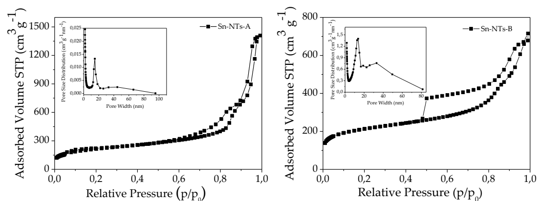
FIGURE 1.2: Nitrogen adsorption/desorption isotherms of Sn-NTs-A and Sn-NTs-B.
