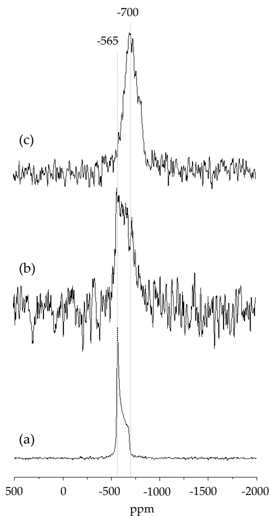
FIGURE 1.4: Solid state 119 Sn static NMR spectra recorded in static conditions of SnO 2 (a), materials Sn-NTs-A (b) and Sn-NTs-B (c).
