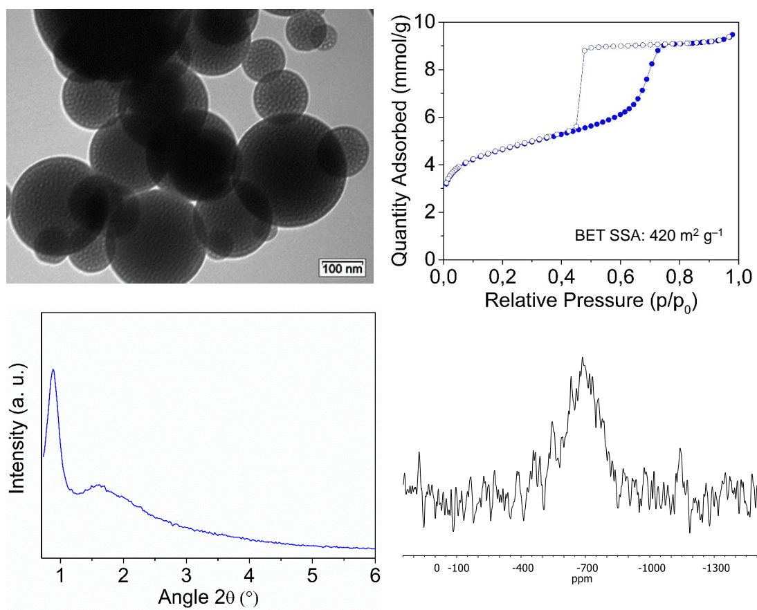
FIGURE A.9: TEM micrograph, nitrogen adsorption/desorption isotherms, Small-angle XRD patterns, 119 Sn static solid state NMR and physicochemical properties summary of Sn-0-F127
