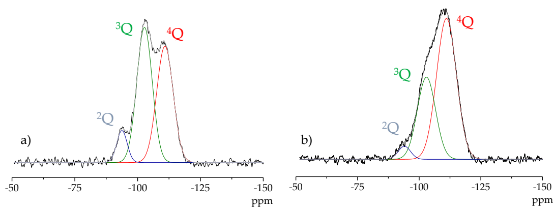
FIGURE 5.8: ^{29}\text{Si} direct excitation MAS NMR spectra of Ga-P-0 calcined at 250\text{ }^\circ\text{C} (top) and 550\text{ }^\circ\text{C} (bottom)
