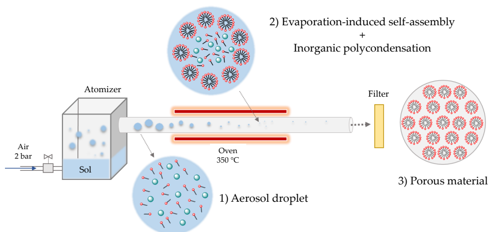
FIGURE 2.1: Schematic view of the aerosol-assisted sol-gel process.
