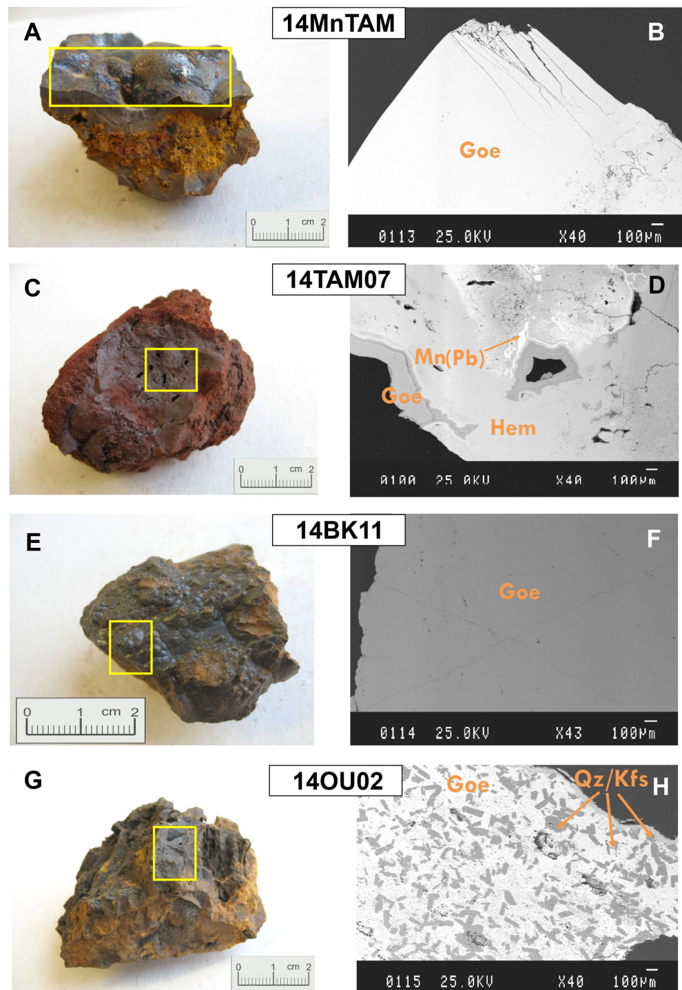
Figure 3. Samples of studied goethite and SEM microphotograph in back-scattered electrons mode, showing the pure character of supergene goethite of the samples 14MnTAM and 14BK11. Goe = goethite; Hem = hematite; Qz = quartz; Kfs = K-feldspar. (A) sample 14MnTAM, (B) SEM microphotograph in back-scattered electrons mode of sample 14MnTAM, (C) sample 14TAM07, (D) SEM microphotograph in back-scattered electrons mode of sample 14TAM07, (E) sample 14BK11, (F) SEM microphotograph in back-scattered electrons mode of sample 14BK11, (G) sample 14OU02, (H) SEM microphotograph in back-scattered electrons mode of sample 14OU02.
