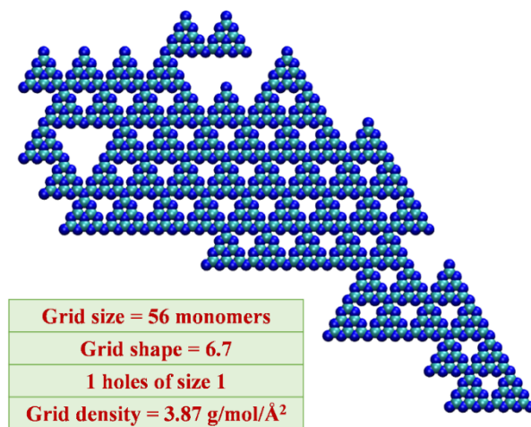
Figure 6. Small g\text{-C}_3\text{N}_4 grid with large shape index obtained from a KMC run carried out with option “ lnl_dir ” at 750 K.
