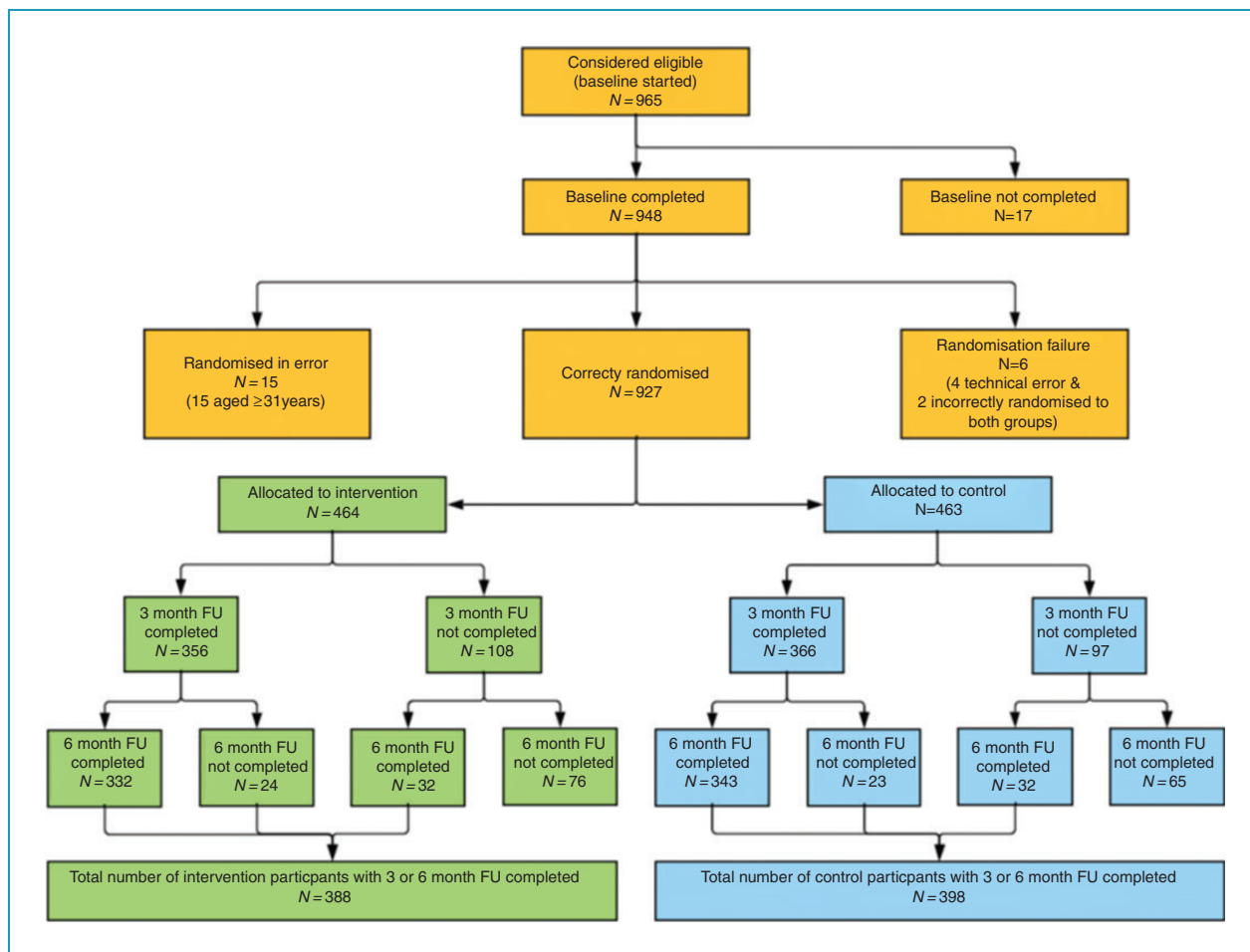
Figure 2. CONSORT diagram.
