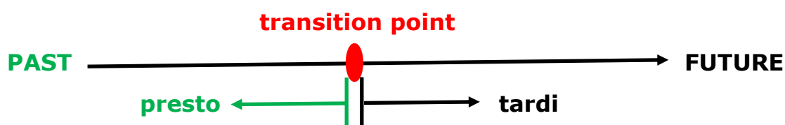
Fig. 10. Transition between the two regions presto – tardi on the time scale.
