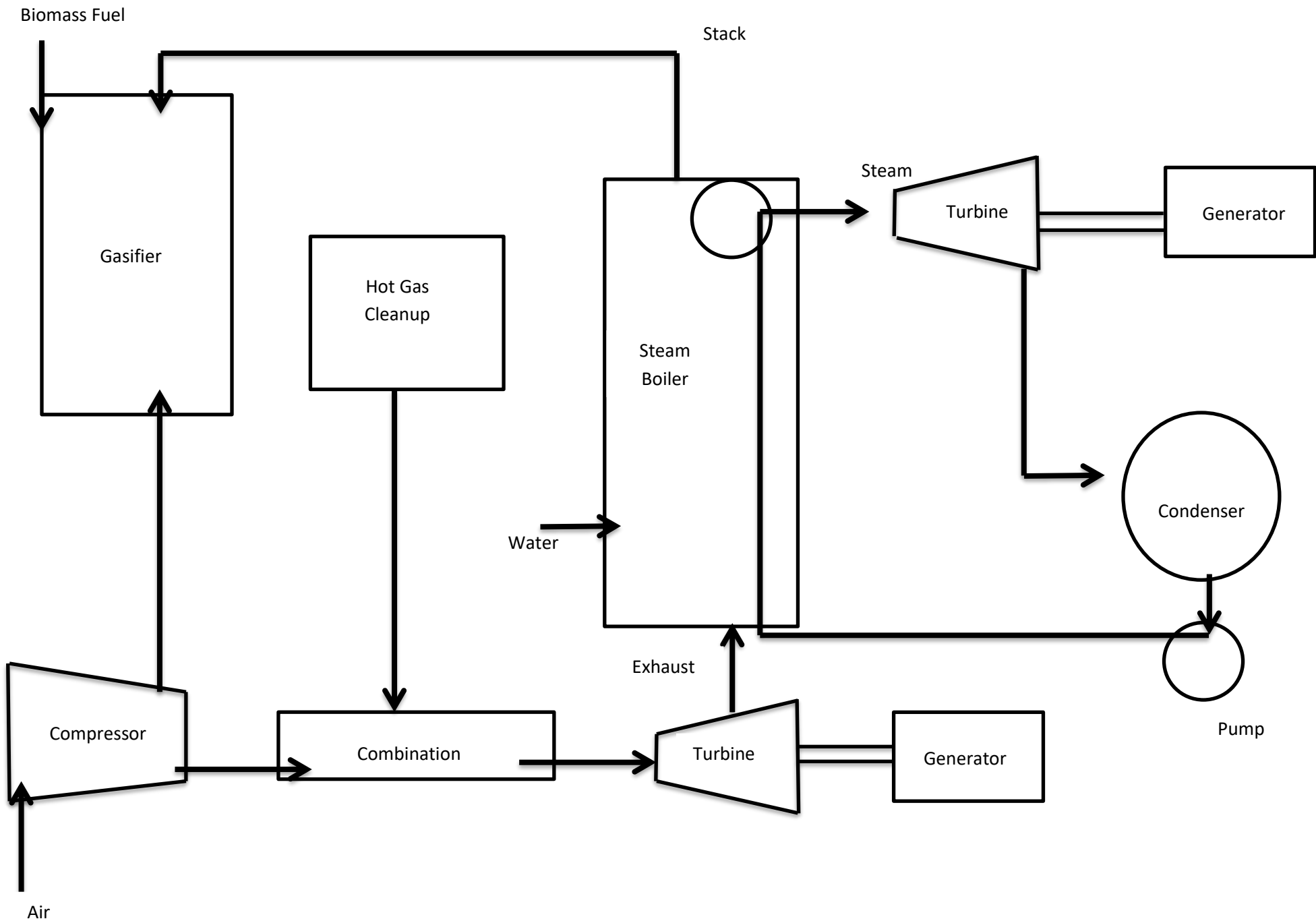
Figure 1. Integrated biomass gas turbine/steam combined cycle power plant (Alidrisi, and Demirbas, 2016)
