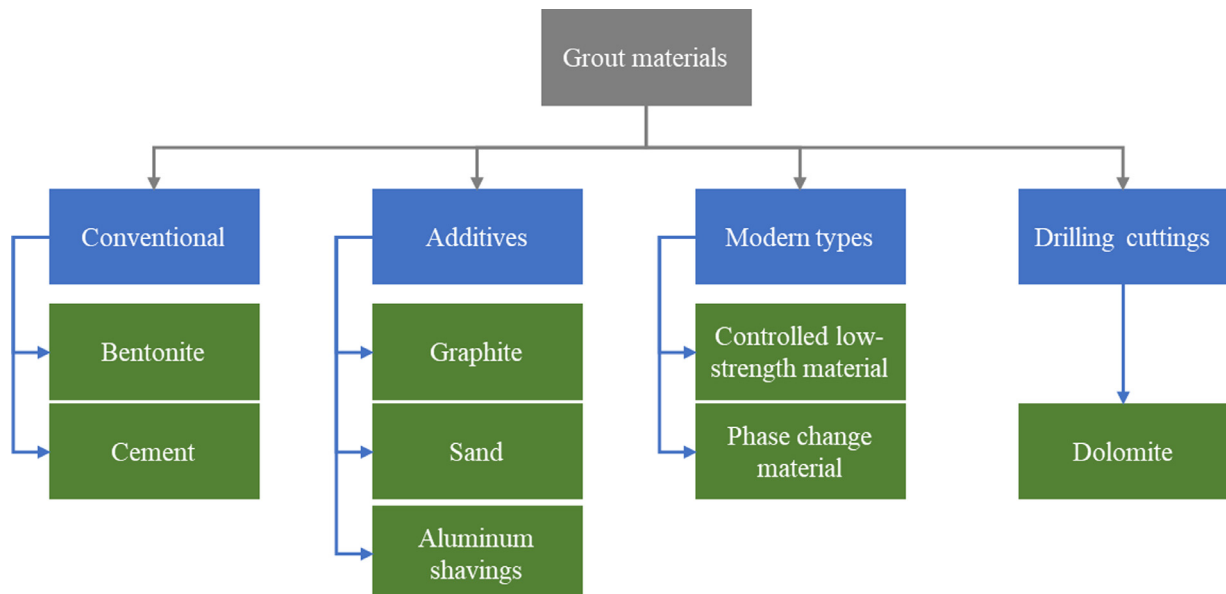
Fig. 3. Commonly used grout materials in geothermal energy systems.
