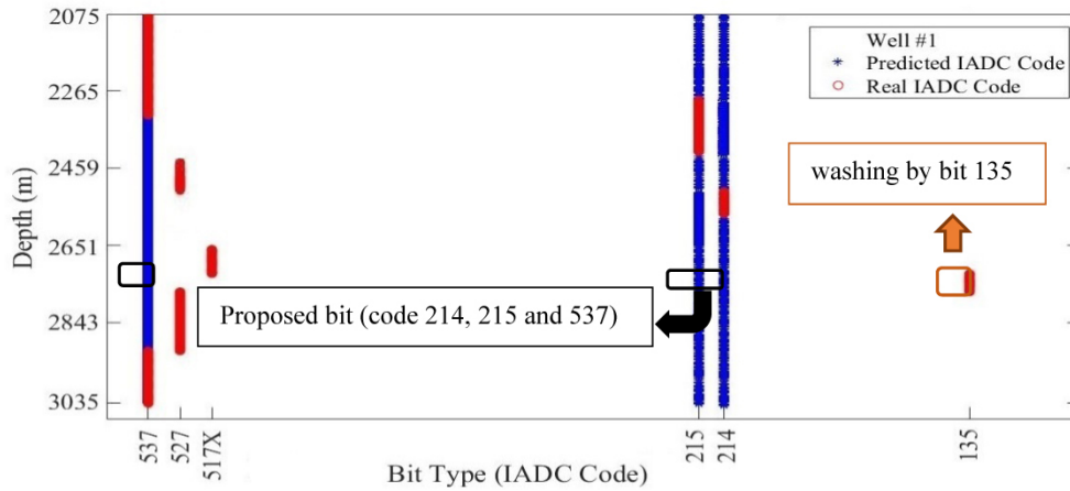
Figure 7: The mismatching between the proposed bits by the Markov chain (code 214, 215, and 537) and the used bit (codes 135) for washing in well #1
