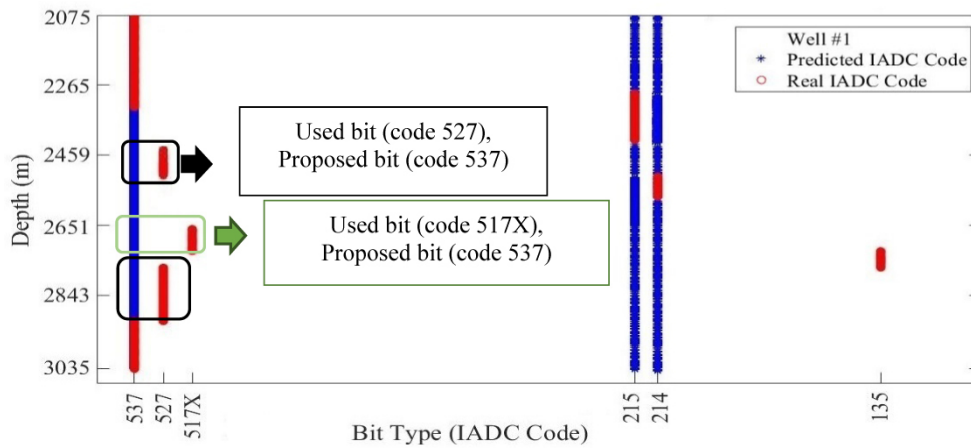
Figure 4: The mismatching between the proposed bit by the Markov chain (code 537) and the improper used bit (codes 527 and 517X) in well #1
