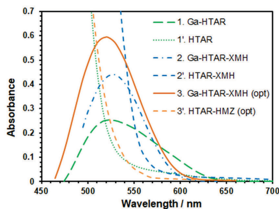
Figure 1. Absorption spectra of complexes against blanks (1–3; c_{\text{Ga}} = 1 \times 10^{-5} mol dm -3 , t_{\text{ex}} = 3 min) and corresponding blanks against chloroform (1'–3').
