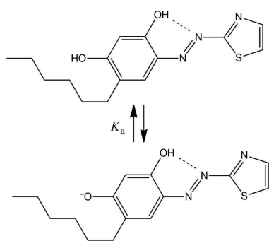
Figure 3. Equilibrium between the two forms of HTAR ( \text{H}_2\text{L} and \text{HL}^- ).
