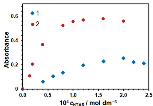
Figure 4. Effect of HTAR concentration in the absence (1) or presence (2) of XMH. (1) c_{\text{Ga}} = 1 \times 10^{-5} mol dm ^{-3} , \text{pH} 6.4 , t_{\text{ex}} = 3 min, \lambda = 523 nm; (2) c_{\text{Ga}} = 1 \times 10^{-5} mol dm ^{-3} , c_{\text{XMH}} = 2 \times 10^{-3} mol dm ^{-3} , \text{pH} 5.0 , t_{\text{ex}} = 3 min, \lambda = 521 nm.
