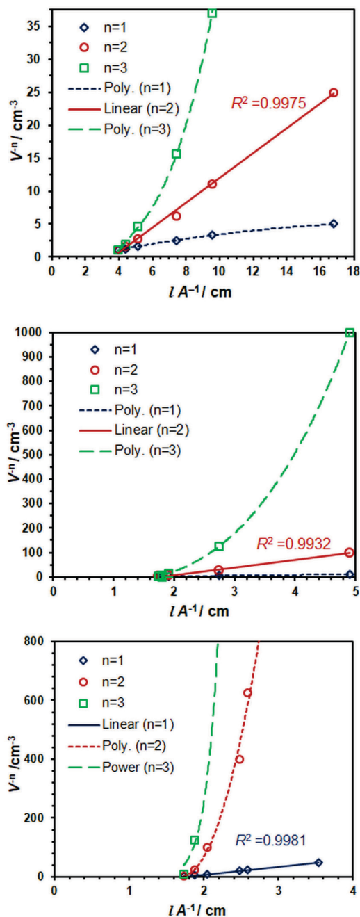
Figure 7. Determination of the HTAR-to-Ga molar ratio in the absence (a) and presence (b) of XMH and the XMH-to-Ga molar ratio (c) by the straight-line method of Asmus. The experimental conditions are given in Figs. 4 and 5, respectively.
