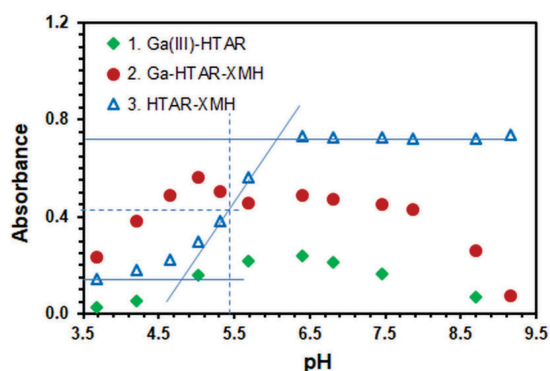
Figure 2. Effect of pH of the aqueous phase on the absorbance ( \lambda = 523 nm). (1) c_{\text{Ga}} = 2 \times 10^{-5} mol dm ^{-3} , c_{\text{TAR}} = 2 \times 10^{-4} mol dm ^{-3} ; (2) c_{\text{Ga}} = 1 \times 10^{-5} mol dm ^{-3} , c_{\text{HTAR}} = 2 \times 10^{-4} mol dm ^{-3} , c_{\text{XMH}} = 2 \times 10^{-3} mol dm ^{-3} ; (3) c_{\text{HTAR}} = 2 \times 10^{-4} mol dm ^{-3} , c_{\text{XMH}} = 2 \times 10^{-3} mol dm ^{-3} .
