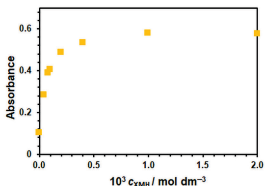
Figure 5. Effect of XMH concentration on the absorbance. c_{\text{Ga}} = 1 \times 10^{-5} mol dm ^{-3} , c_{\text{HTAR}} = 1.4 \times 10^{-4} mol dm ^{-3} , \text{pH} 5.0 , t_{\text{ex}} = 3 min, \lambda = 521 nm.
