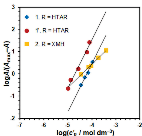
Figure 6. Determination of the HTAR-to-Ga molar ratio in the absence (1) and presence (1') of XMH and the XMH-to-Ga molar ratio (2) by the mobile equilibrium method. The experimental conditions are given in Figs. 4 and 5, respectively. Straight-line equations: (1) y = 2.2x + 9.1 , R^2 = 0.9923 ; (1') y = 2.2x + 10.1 , R^2 = 0.9860 ; (2) y = 1.04x + 4.6 , R^2 = 0.9971 .
