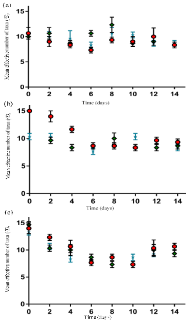
Figure 5: Consortia richness, as determined by the Hill number {}^0D , associated with pH 6.5 (a), 7.0 (b) and 7.5 (c) at {}^{\circ}\text{C} 35 following triplicate incubation in the dark for 14 days and with 0.5 ( \bullet ), 5 ( \blacklozenge ) and 50 ( \star ) mM o -xylene. Each datum point is the mean of triplicate samples. Error bars are SEM.
