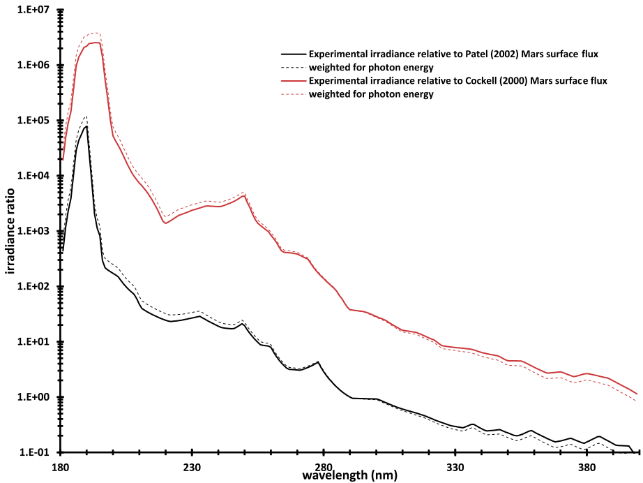
Fig. 11 Quantified relative irradiance of the UV experiment compared to two scenarios at the surface of Mars (see Sect. 4.3 text for scenarios). Ratio of lamp irradiance ( \text{W}/(\text{m}^2 \text{nm}) ) versus the published scenario
