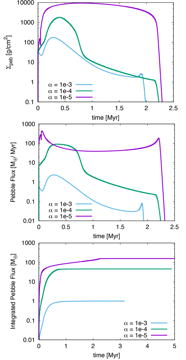
Fig. 5. Evolution of the pebble surface density (top), the pebble flux (middle) and the integrated pebble flux (bottom) of the disc with M_{d,0} = 0.06 M_{\odot} of the nominal set-up (Fig. 3). The pebble flux ceases once the gap due to photoevaporation is carved at a \approx 3-4 au (see Fig. 1).
