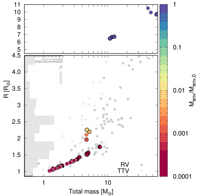
Fig. 11. Final mass-radius for all the planets with P < 100 days and M_{core} \geq 1 M_{\oplus} , represented by black-border colored circles. The grey-border colored circles represent the planets computed with low dust opacity (Sect.4.2). The colors show the final envelope mass relative to the initial one. The final mass of the envelope and radii are computed following Sec. 2.7. The grey small dots/triangles represent the RV/TTV planets used by Zeng et al. (2019) (from their Fig.2 and Table S1) and were used to construct the grey histogram on the left, which depicts the percentage of planets as a function of their radius.
