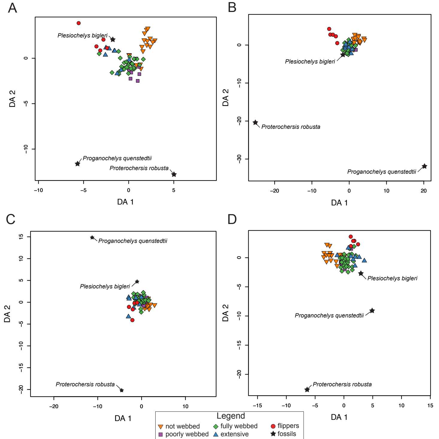
Figure 8 Results of the phylogenetic flexible discriminant analysis (pFDA) based on four different dataset configurations. (A) All landmarks and curves, SET1. (B) Outline of the carapace, SET2. (C) Transverse cross-section, SET3. (D) Longitudinal cross-section, SET4. Complete data are available in Table S5.
