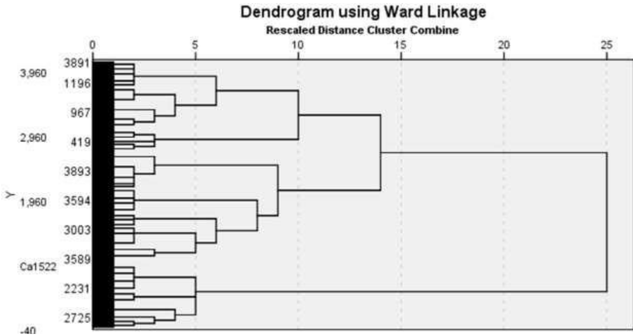
4-1. Dendrograms derived from Ward cluster analysis
