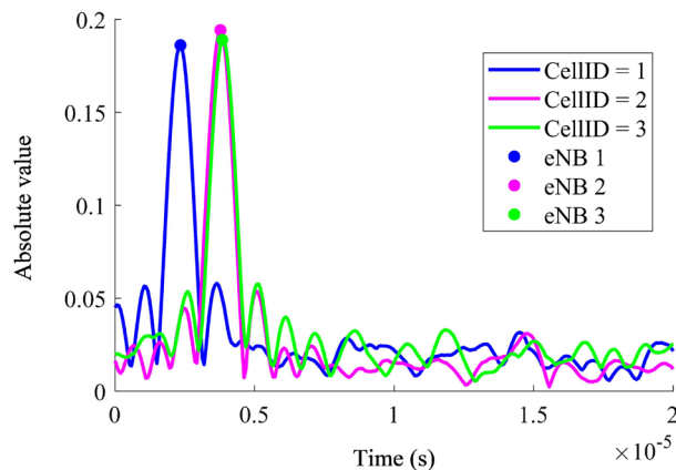
Fig. 7. Correlation profile for ToA estimation
