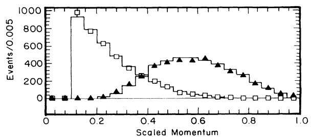
FIG. 1. Distribution in the lower and higher scaled momentum per event for data (open squares and solid triangles, respectively) and Monte Carlo simulation (histogram) of the detected electrons.
