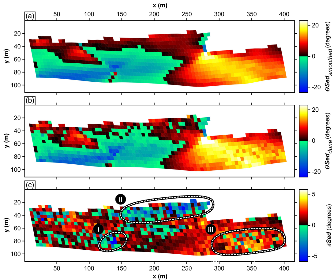
Figure 9. Planform sediment transport directions (calculated using Equations 11a–11d) for (a) the Smoothed DEM simulation ( \theta_{Sed\_smoothed} ) and (b) the Dune DEM simulation ( \theta_{Sed\_dune} ). Calculations were performed at fine resolution and then spatially averaged over a 5 m grid. Zero is downstream. Positive and negative directions are toward the true left and right banks, respectively. (c) Deviation between the sediment transport directions for the Dune DEM simulation and the Smoothed DEM simulation ( \delta_{Sed} ; calculated using Equation 12), spatially averaged at 5 m resolution. Results have been calculated and are shown, only for the sand-bedded regions of the channel.
