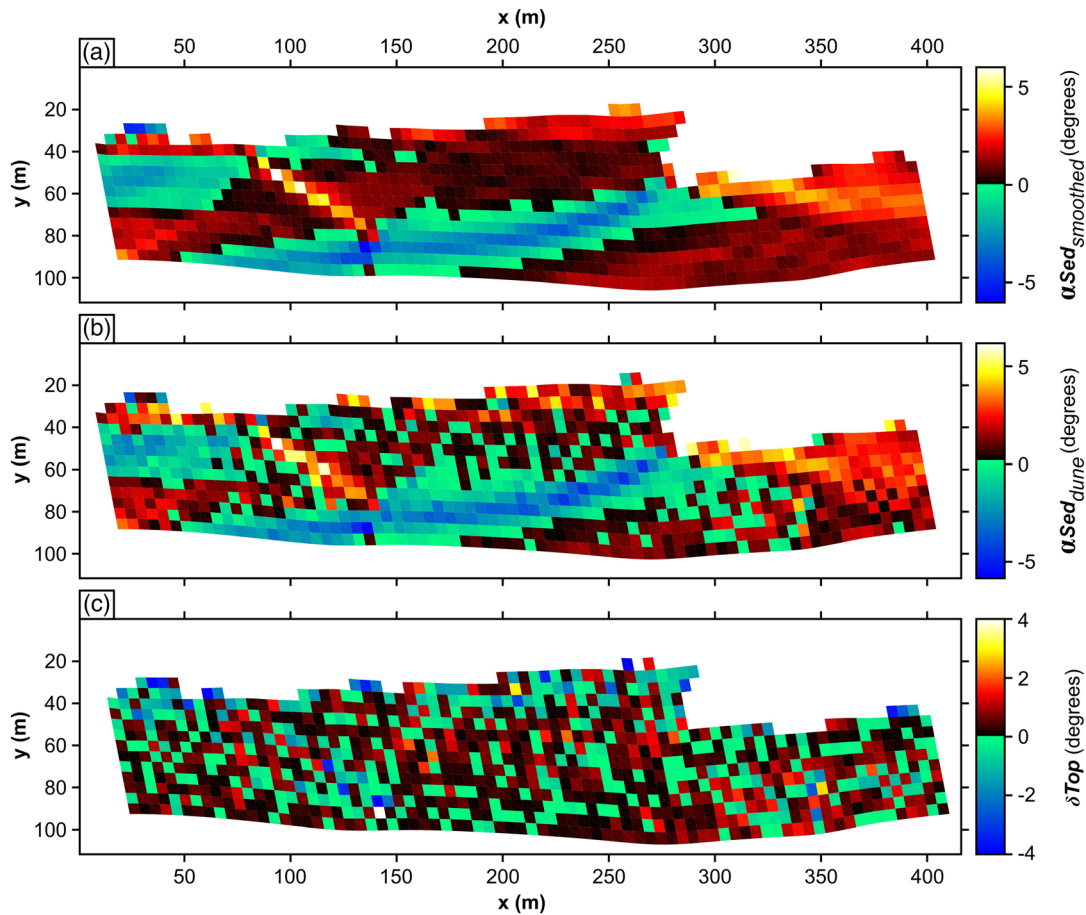
Figure 11. Planform patterns of the deviation between the sediment transport direction and the near-bed flow direction calculated for (a) the Smoothed DEM simulation ( \alpha_{Sed\_smoothed} = \theta_{Sed\_smoothed} - \theta_{NBF\_smoothed} ) and (b) the Dune DEM simulation ( \alpha_{Sed\_dune} = \theta_{Sed\_dune} - \theta_{NBF\_dune} ), shown at 5 m resolution for the sand bed portion of the reach. (c) Planform patterns of the difference ( \delta Top ; calculated using Equation 14) between values of (\theta_{Sed} - \theta_{NBF}) for the Dune DEM and Smoothed DEM simulations, shown at 5 m resolution for the sand bed portion of the reach.
