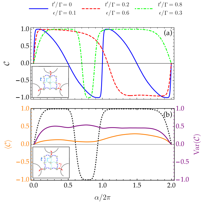
FIG. 9. Heat circulation with a square central structure. (a) Circulation coefficient for t = 0.5\Gamma and various combinations of t' and \epsilon . (b) Ensemble-averaged \langle \mathcal{C} \rangle (solid orange line), for a random variation of the parameters, compared with the corresponding result when no sample-to-sample variation is present (dashed black curve). The solid purple line shows the variance of \mathcal{C} .
