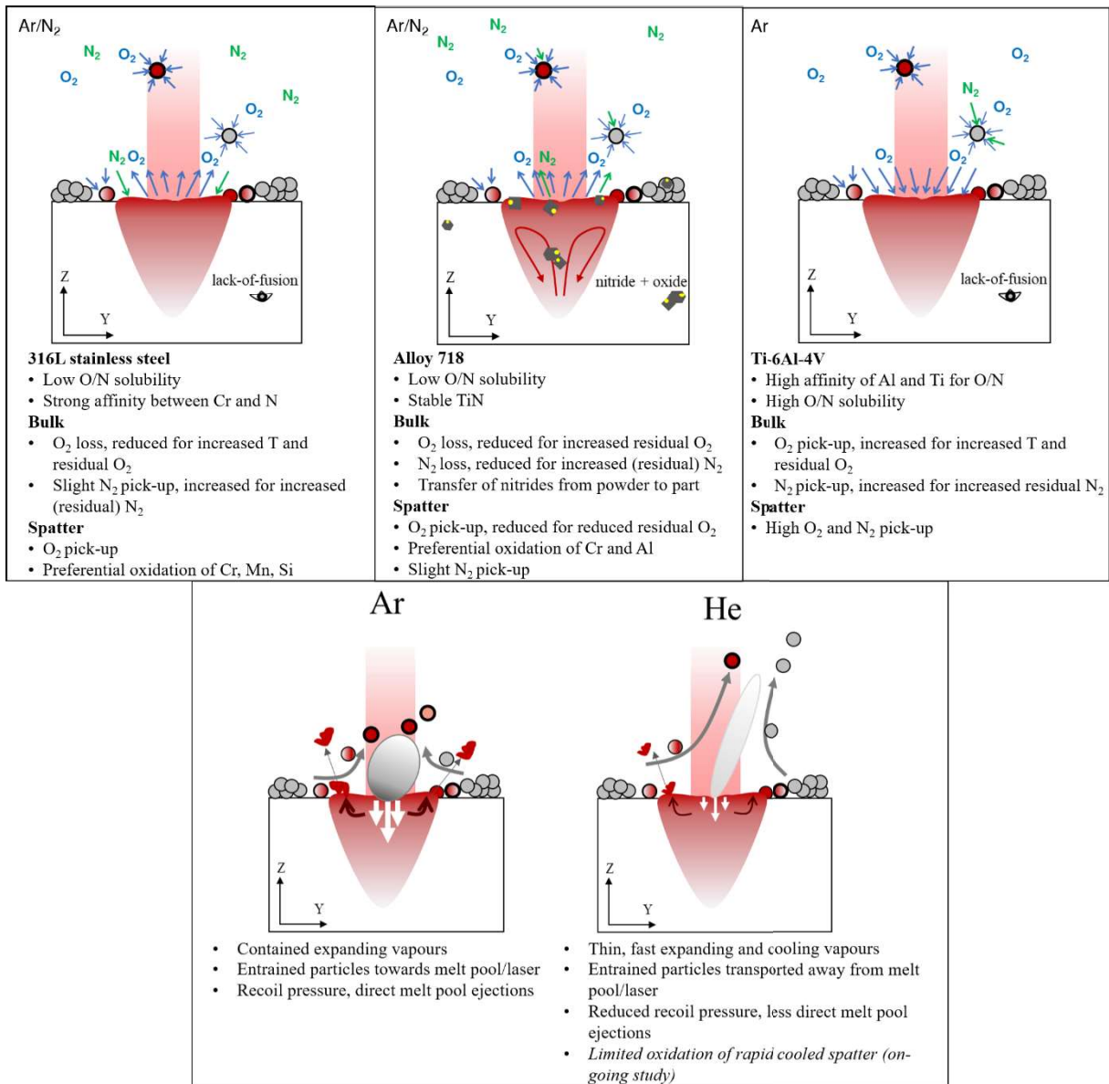
Figure 28: Summarizing illustrations of findings connected to oxygen and nitrogen exchange during L-PBF and model of the effect of helium addition on the melt pool dynamics.
