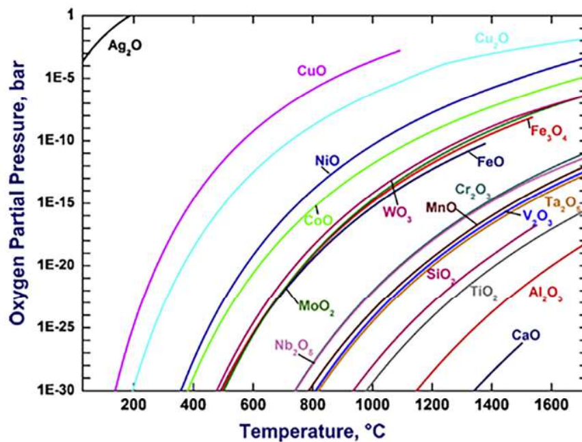
Figure 9: Equilibrium partial pressure of oxygen for some oxide/metal systems (plotted with HSC Chemistry) 37 .
