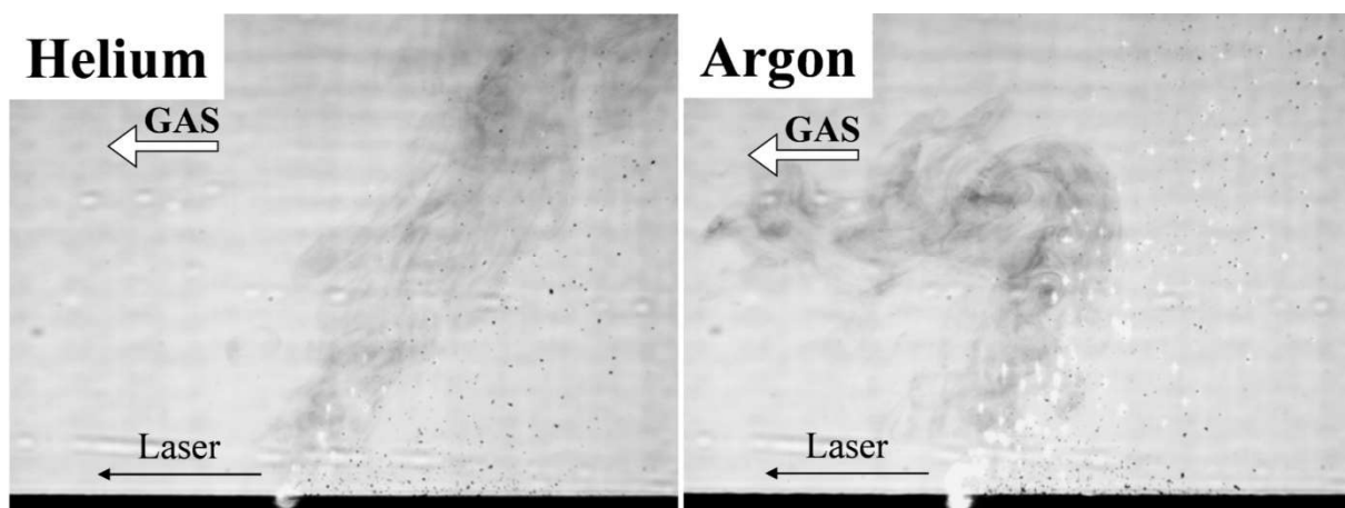
Figure 26: Reduction of Ti-6Al-4V spatter generation using helium, observed on a laboratory-scale L-PBF system (AconityMINI at Fraunhofer ILT, Germany).
